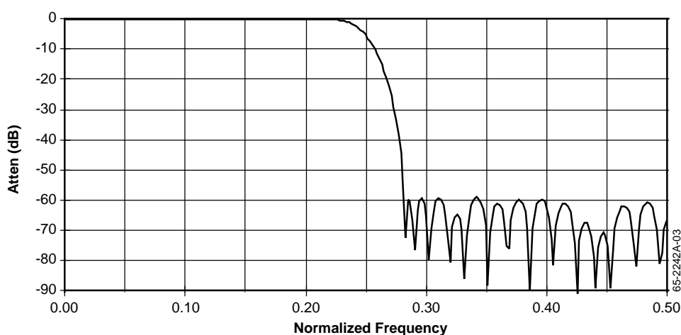
Figure 1. Frequency Response
