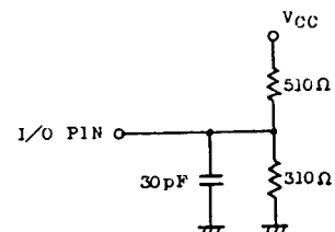
Fig.1 OUTPUT LOAD
