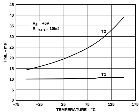
Figure 4. T1 and T2 Times vs. Temperature
