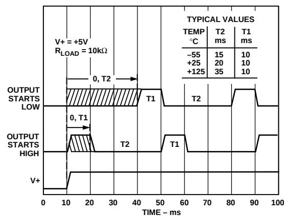
Figure 16. Start-Up Response
