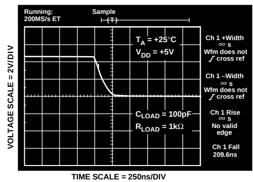
Figure 5. TMP03 Output Fall Time at +25°C
