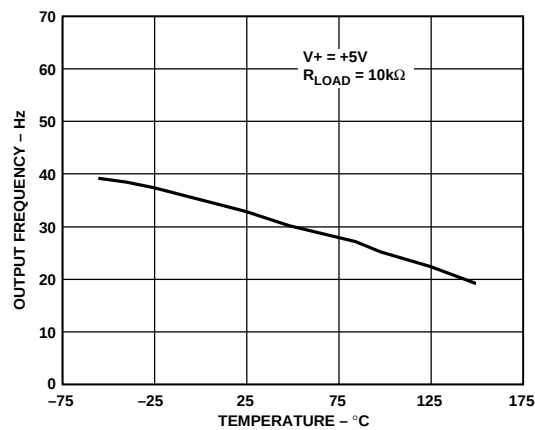
Figure 3. Output Frequency vs. Temperature
