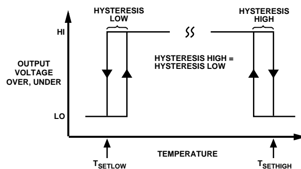
Figure 17. TMP12 Hysteresis Profile
