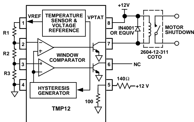
Figure 23. Reed Relay Drive
