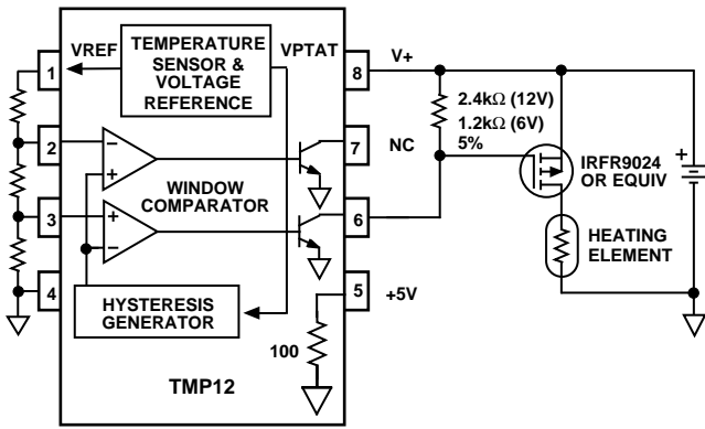
Figure 24. Driving a P-Channel MOSFET
