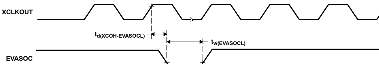
Figure 6–15. EVASOC Timing
