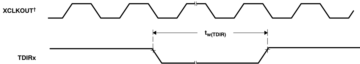
Figure 6–14. TDIRx Timing
