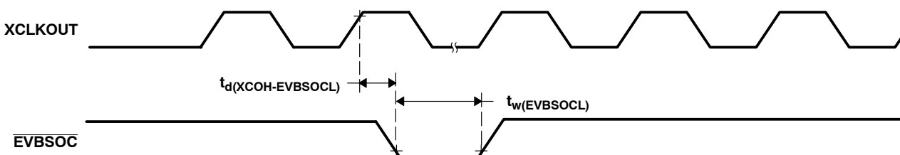
Figure 6–16. EVBSOC Timing
