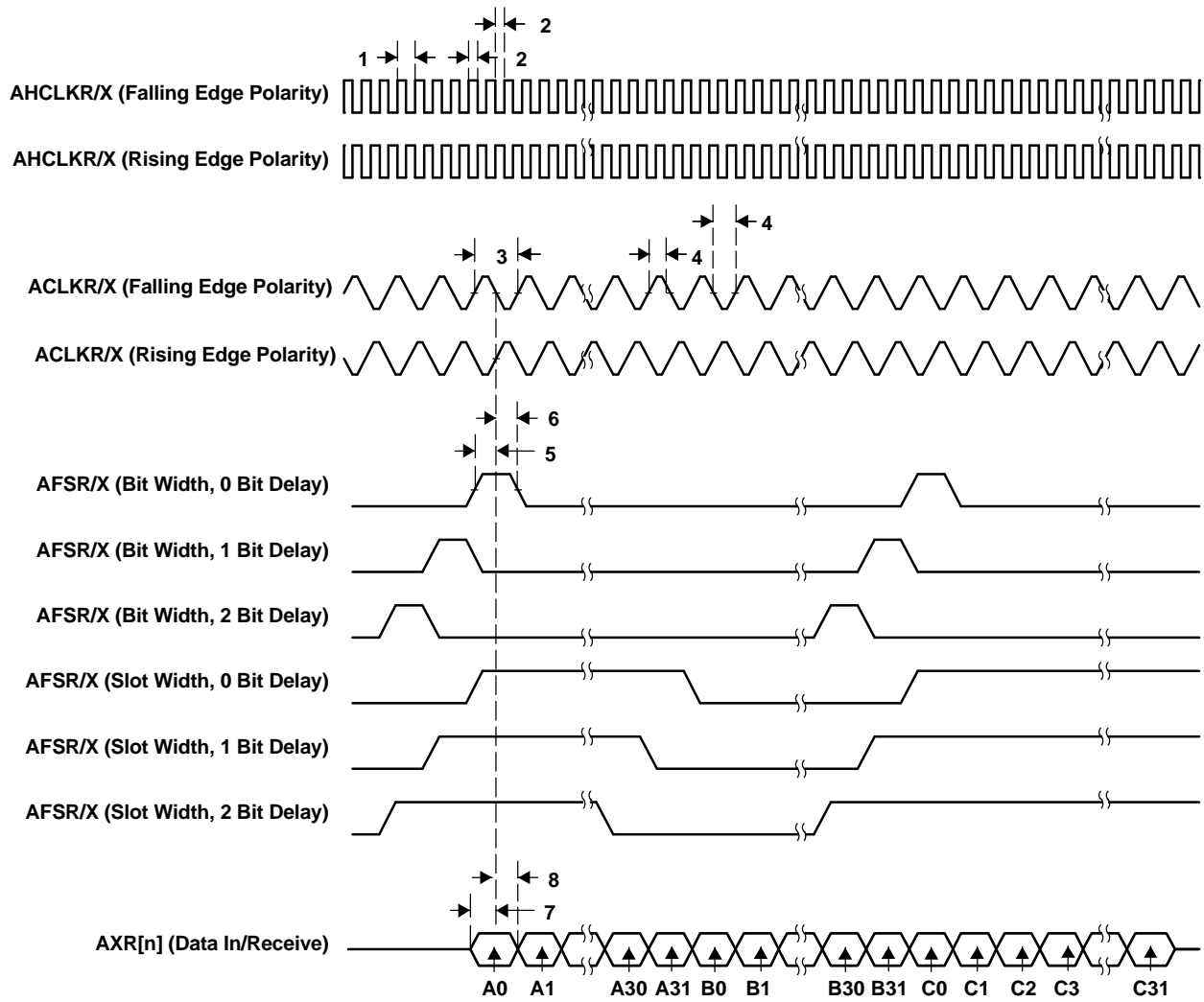
Figure 4-30. McASP Input Timings
