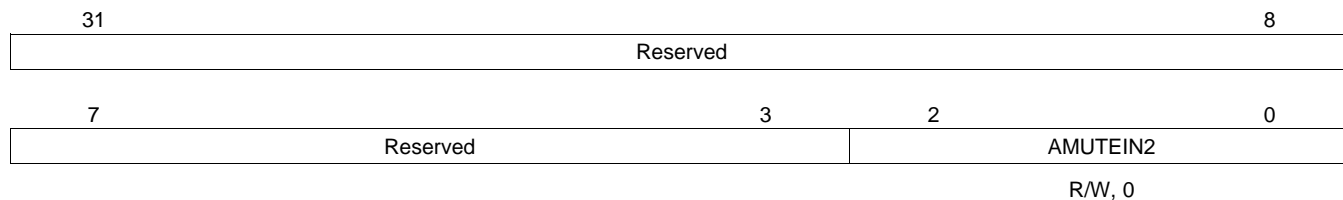
Figure 4-29. CFGMCASP2 Register Bit Layout (0x4000 0020)
