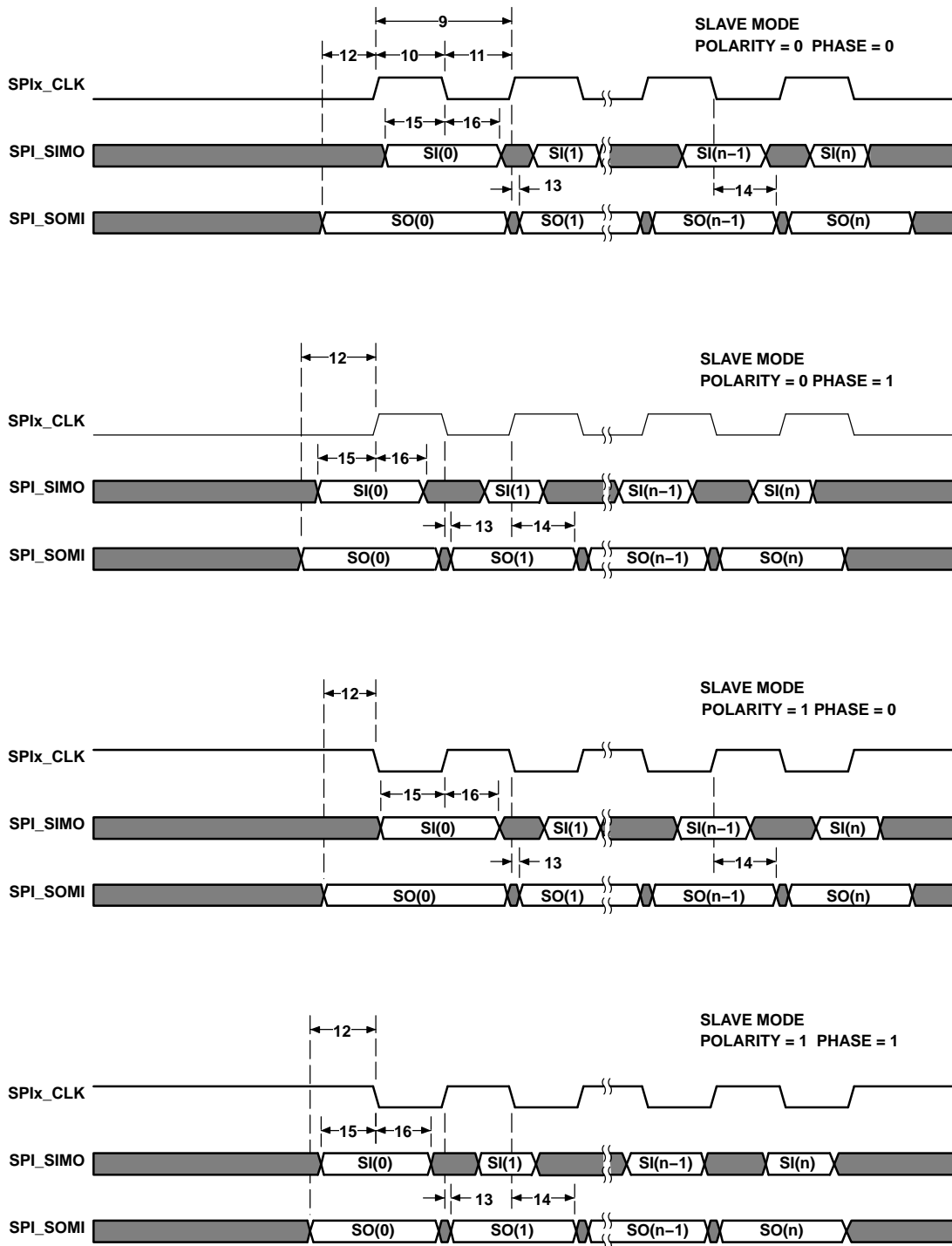
Figure 4-35. SPI Timings—Slave Mode
