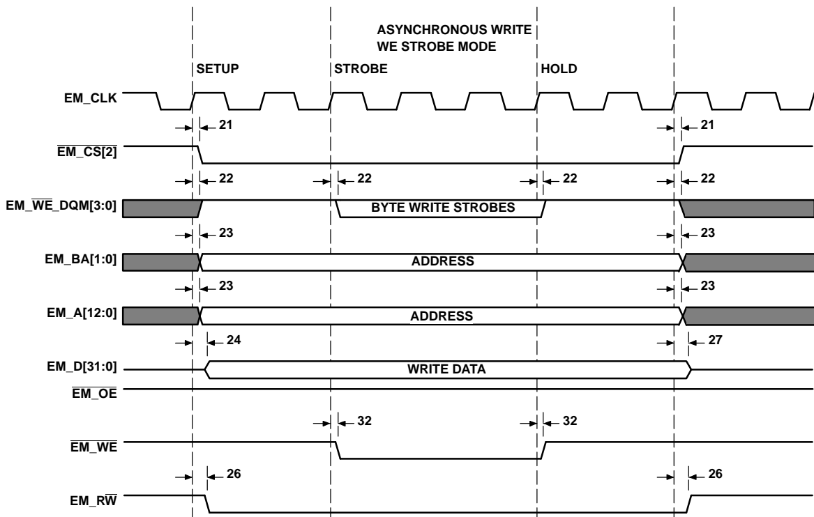
Figure 4-12. Asynchronous Write WE Strobe Mode
