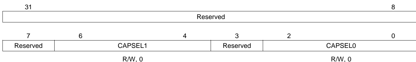
Figure 4-42. CFGRTI Register Bit Layout (0x4000 0014)
