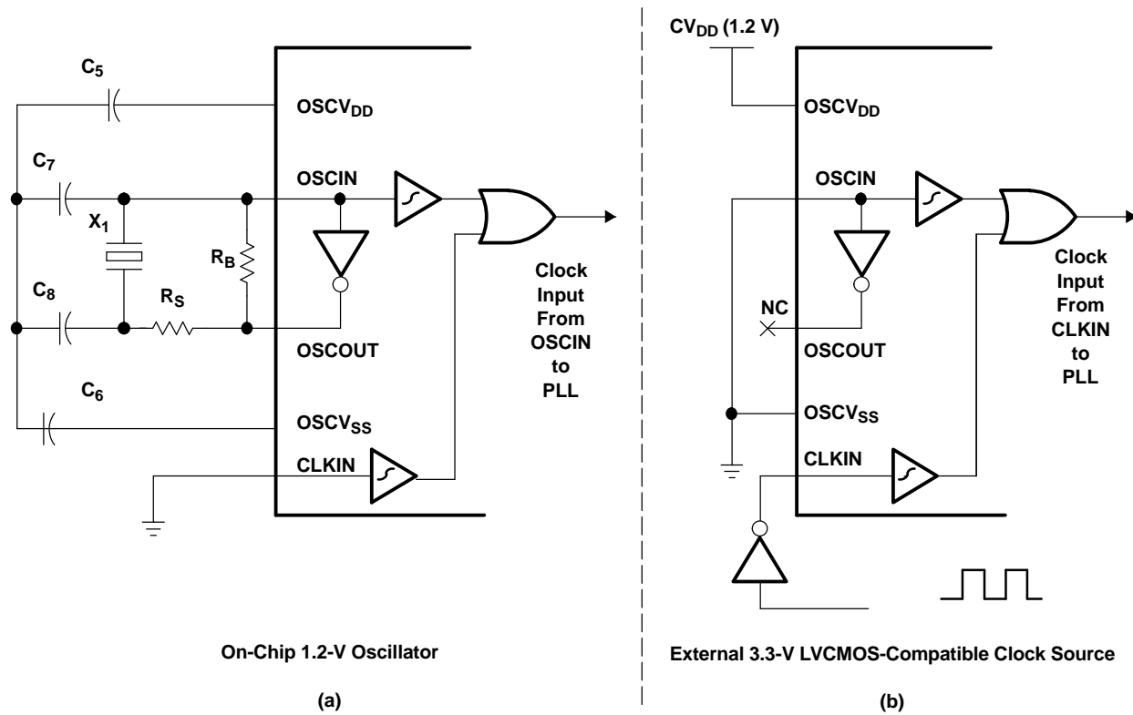
Figure 4-43. C672x Clock Input Options
