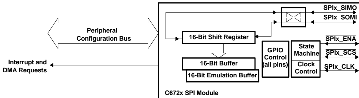
Figure 4-32. Block Diagram of SPI Module
