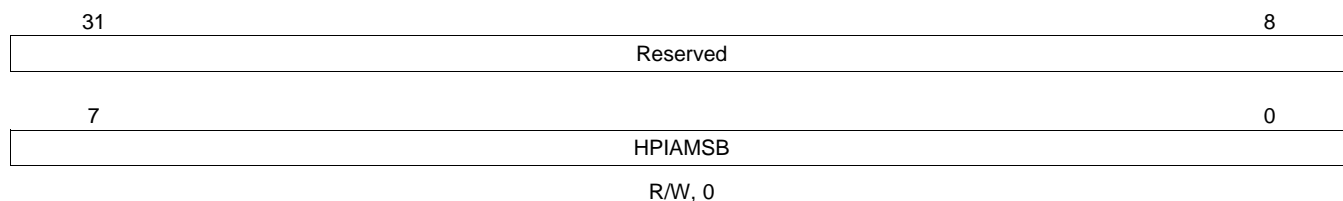
Figure 4-20. CFGHPIAMSB Register Bit Layout (0x4000 000C)
