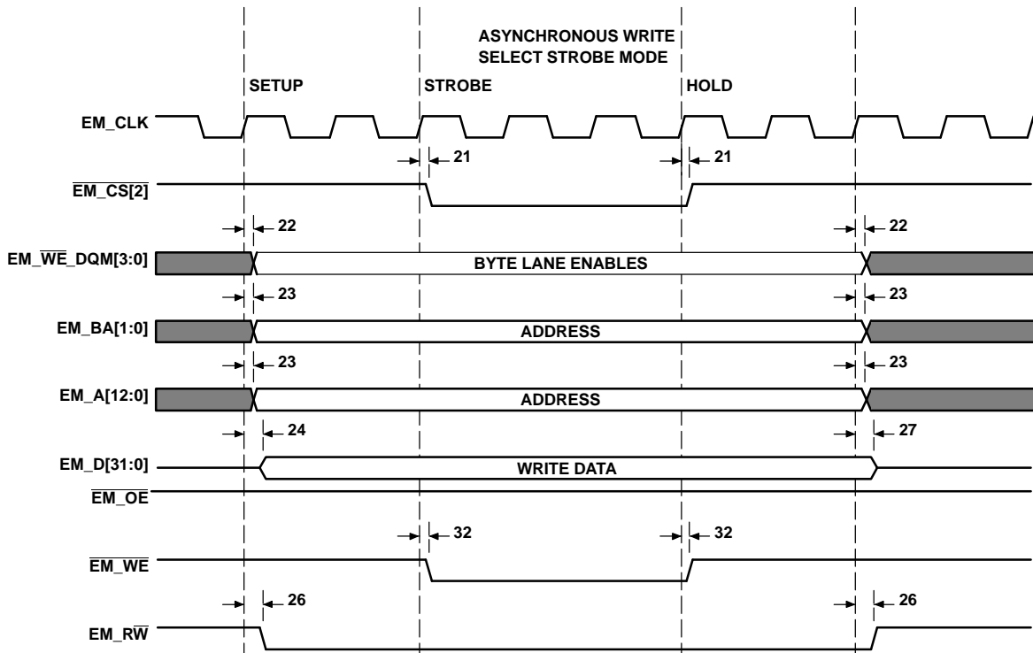
Figure 4-13. Asynchronous Write Select Strobe Mode
