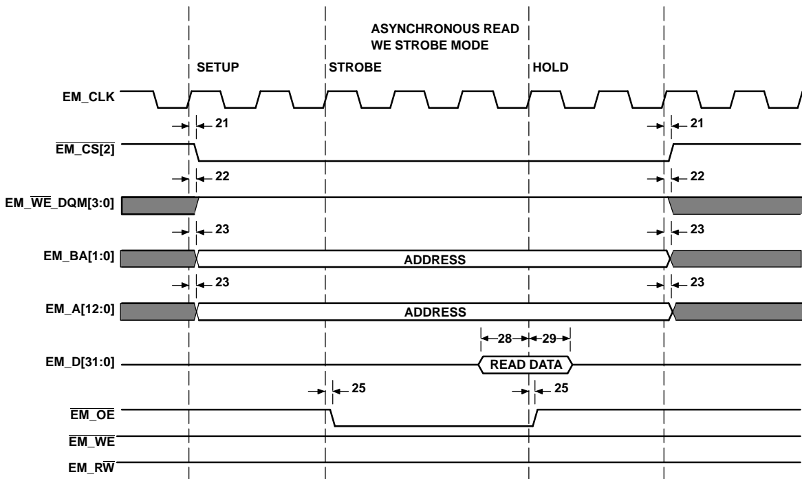
Figure 4-10. Asynchronous Read WE Strobe Mode
