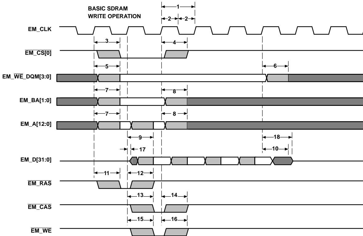
Figure 4-8. Basic SDRAM Write Operation
