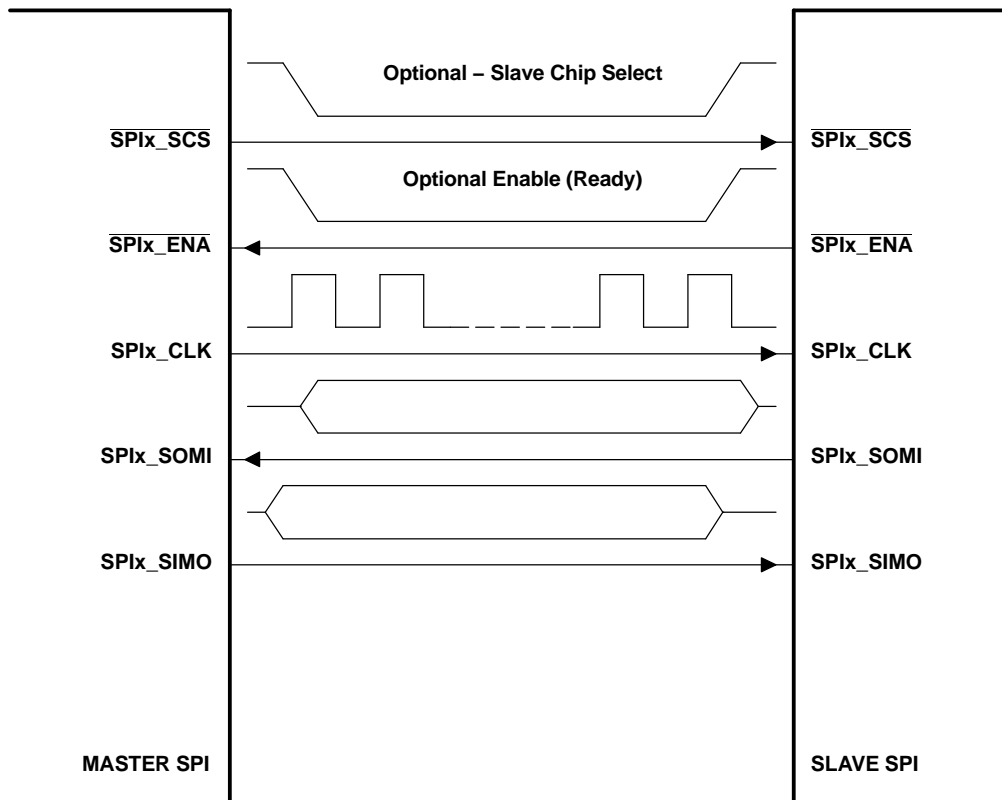
Figure 4-33. Illustration of SPI Master-to-SPI Slave Connection
