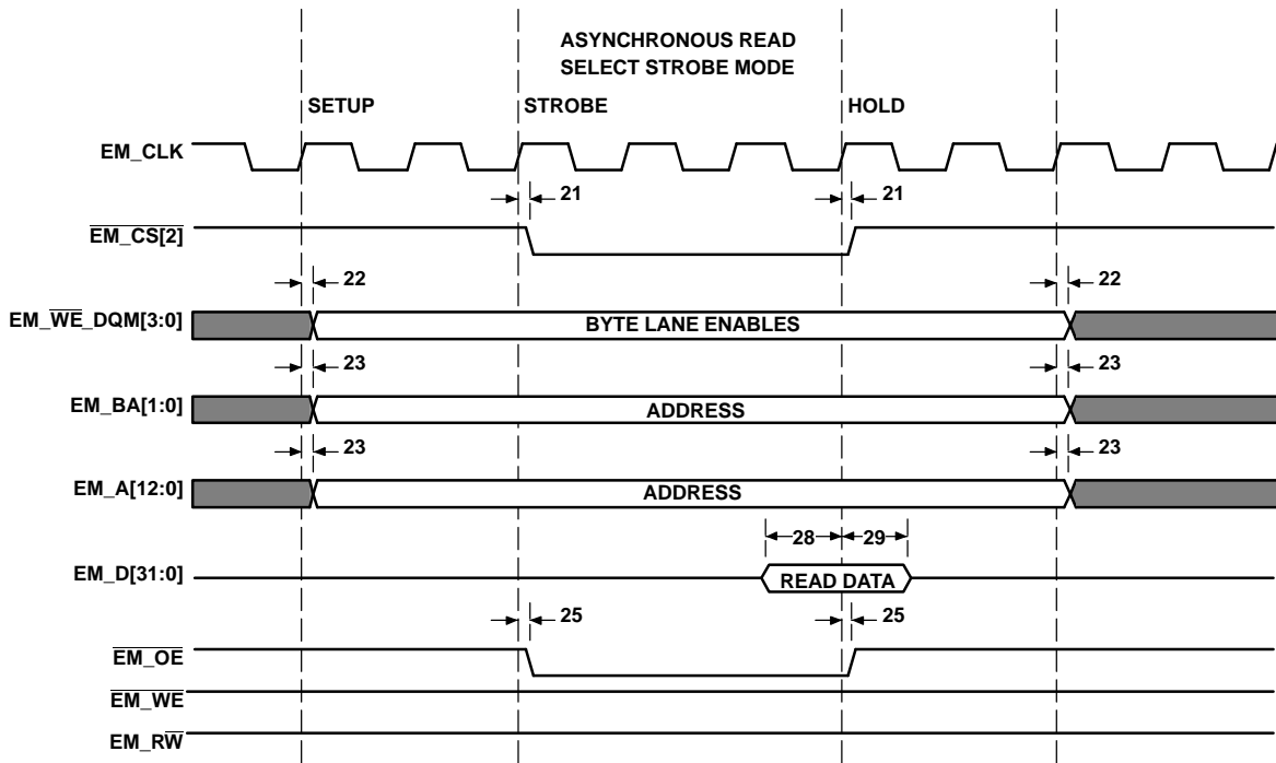
Figure 4-11. Asynchronous Read Select Strobe Mode
