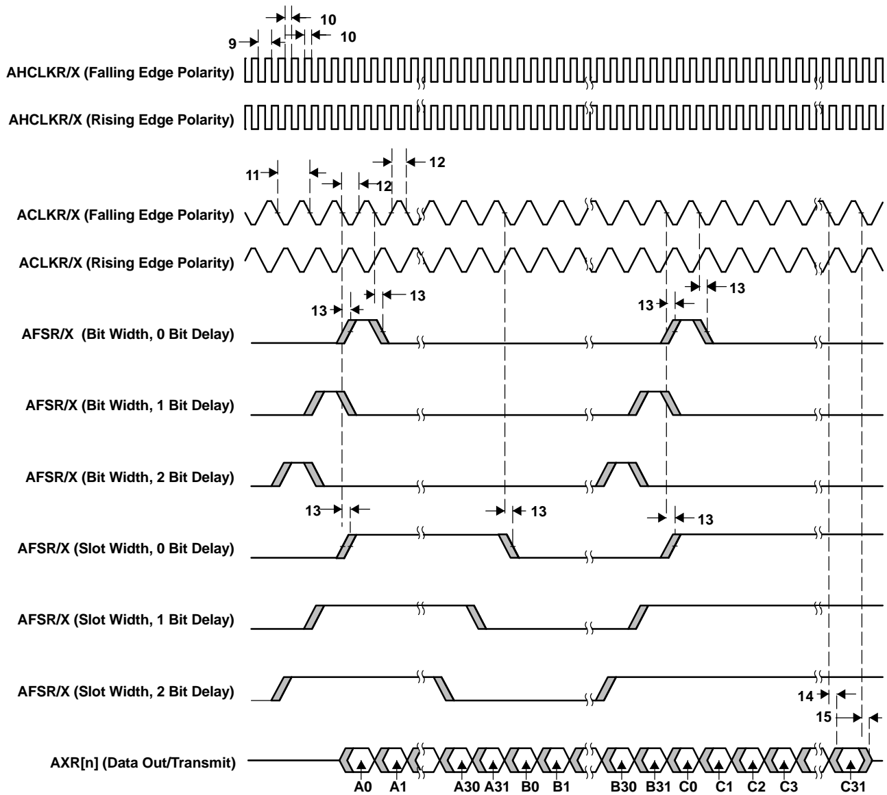
Figure 4-31. McASP Output Timings
