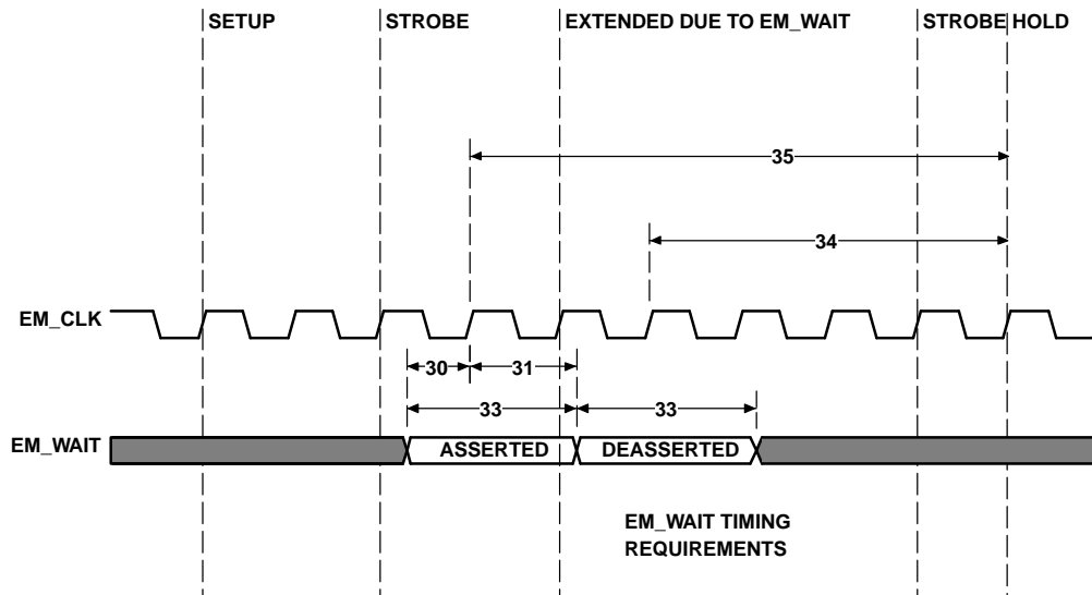
Figure 4-14. EM_WAIT Timing Requirements
