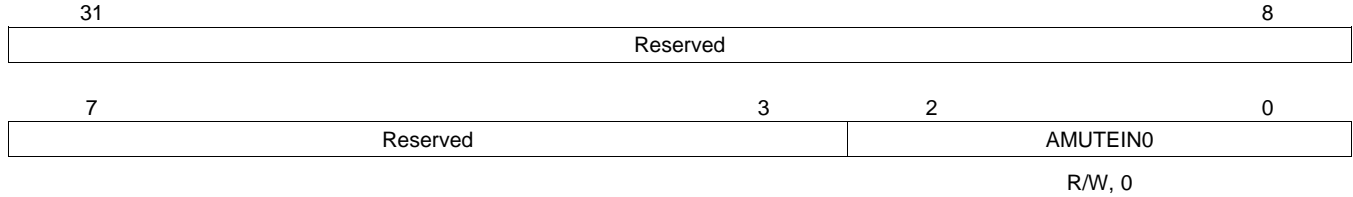
Figure 4-27. CFGMCASP0 Register Bit Layout (0x4000 0018)
