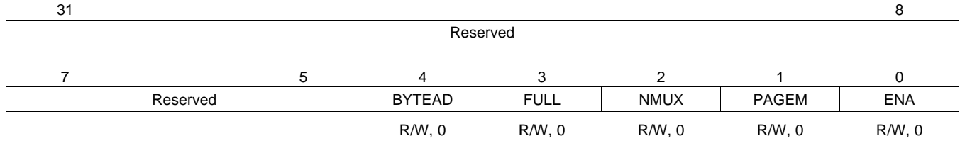
Figure 4-19. CFGHPI Register Bit Layout (0x4000 0008)
