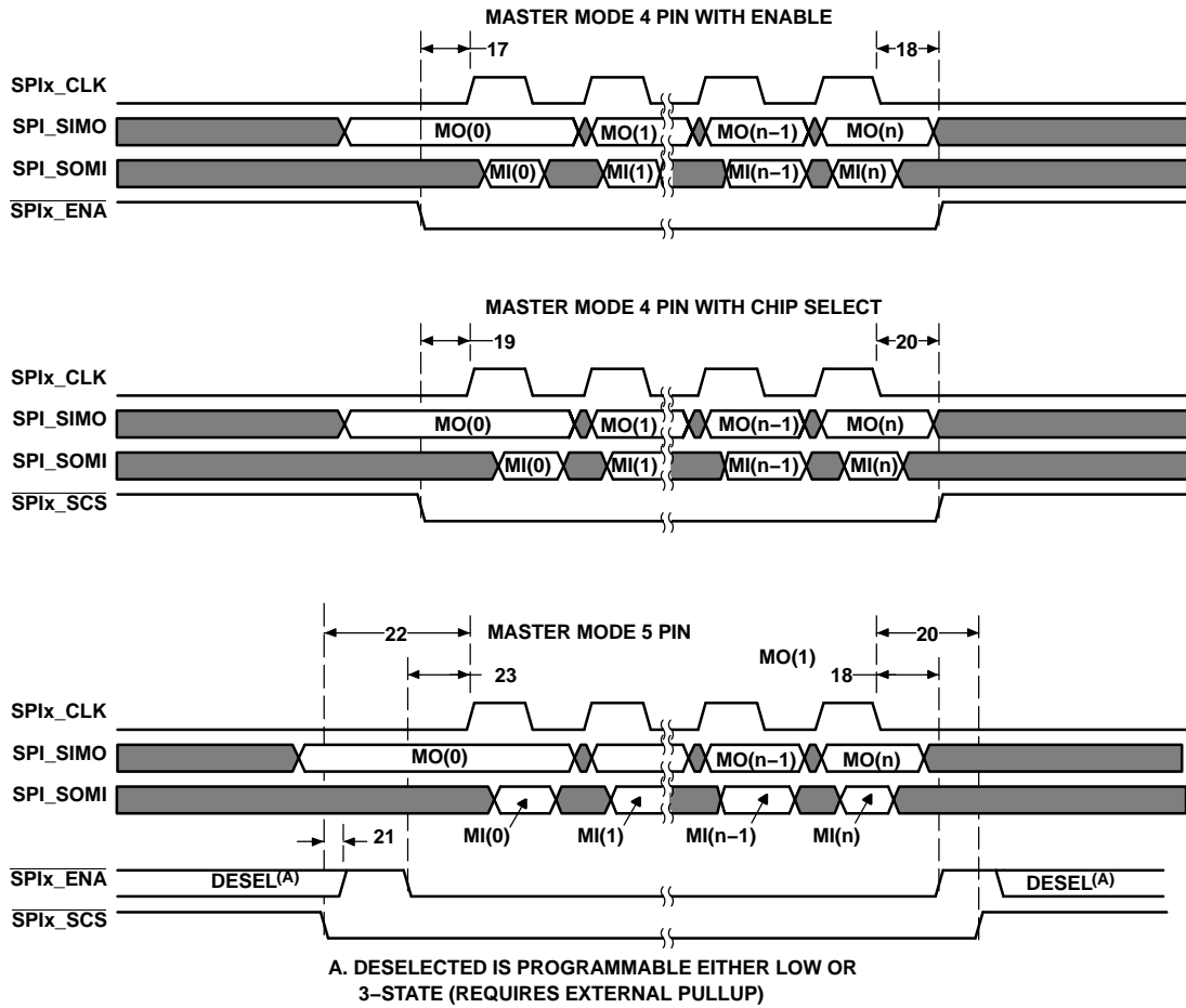
Figure 4-36. SPI Timings—Master Mode (4-Pin and 5-Pin)
