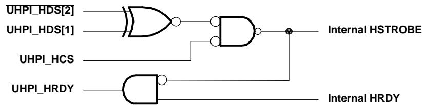
Figure 4-15. UHPI Strobe and Ready Interaction
