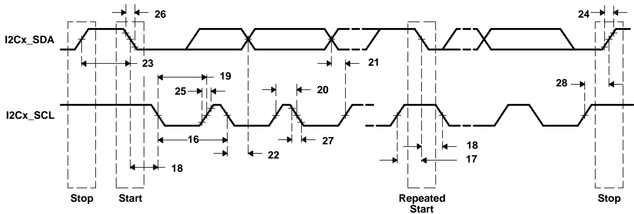
Figure 4-40. I2C Transmit Timings
