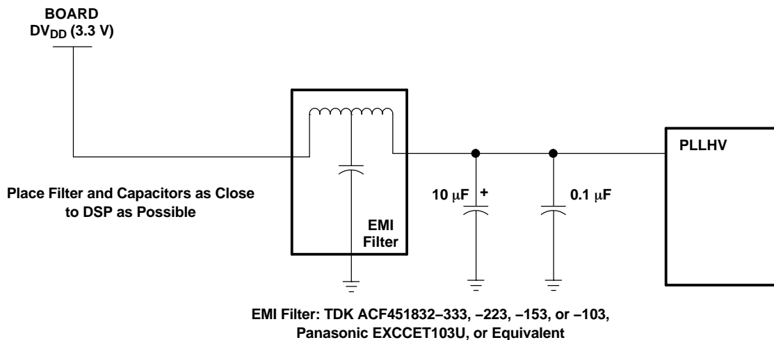
Figure 4-45. PLL Power Supply Filter
