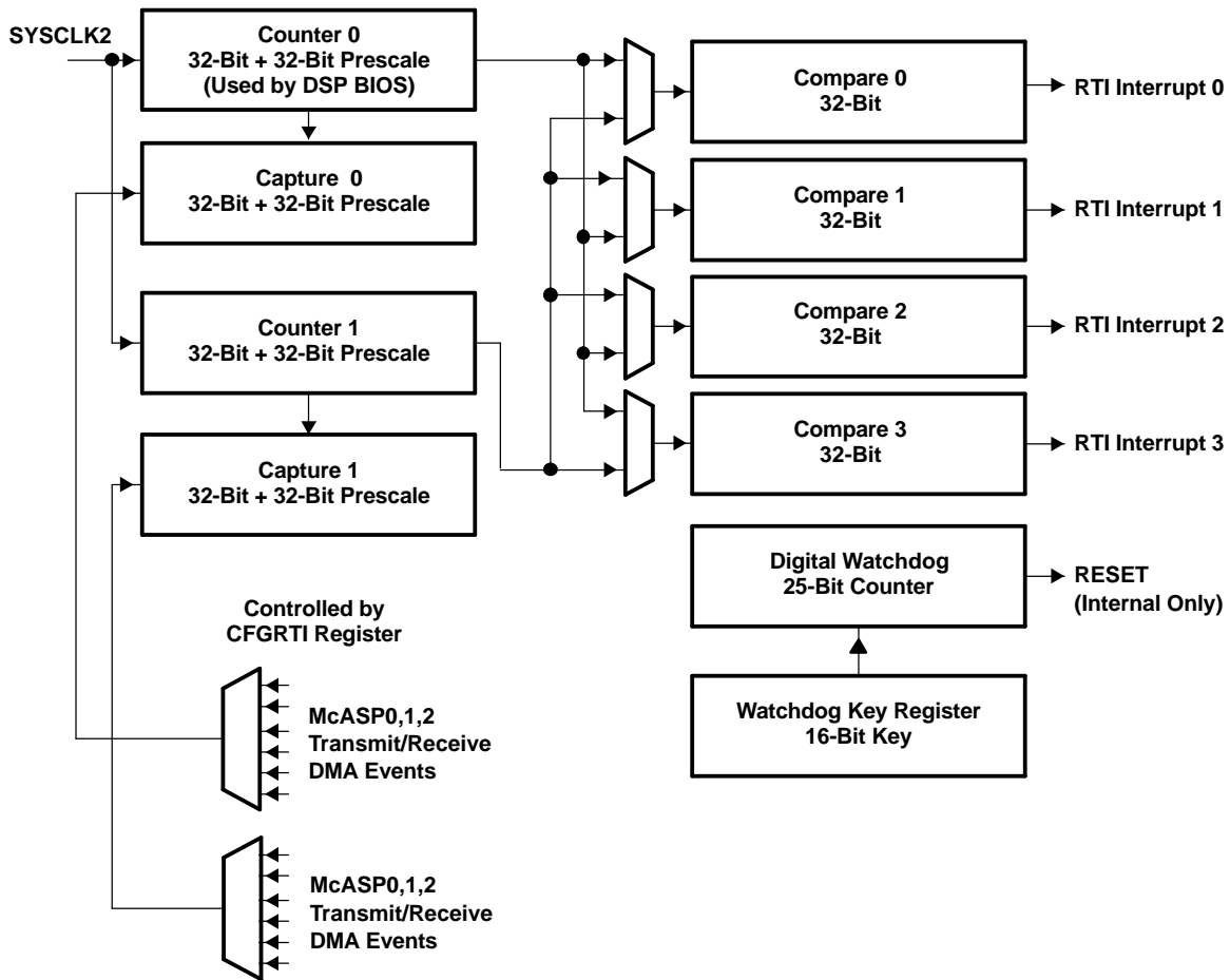
Figure 4-41. RTI Timer Block Diagram
