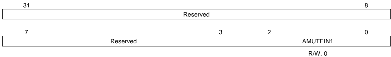
Figure 4-28. CFGMCASP1 Register Bit Layout (0x4000 001C)
