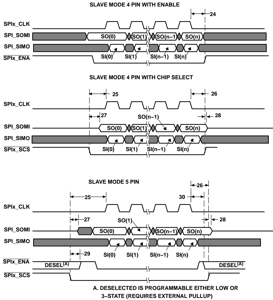
Figure 4-37. SPI Timings—Slave Mode (4-Pin and 5-Pin)
