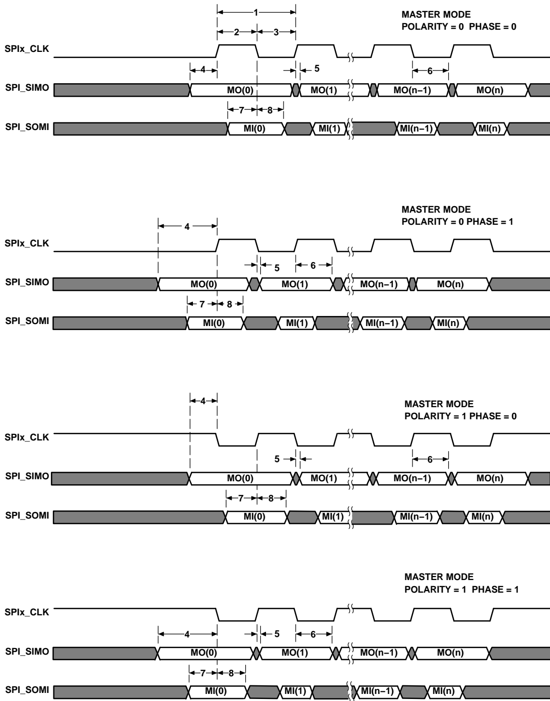
Figure 4-34. SPI Timings—Master Mode
