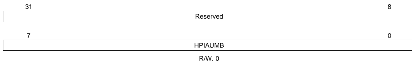
Figure 4-21. CFGHPIAUMB Register Bit Layout (0x4000 0010)
