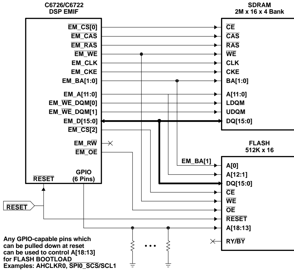
Figure 4-6. C6726/C6722 DSP 16-Bit EMIF Example
