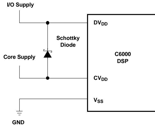
Figure 4-4. Schottky Diode Diagram
