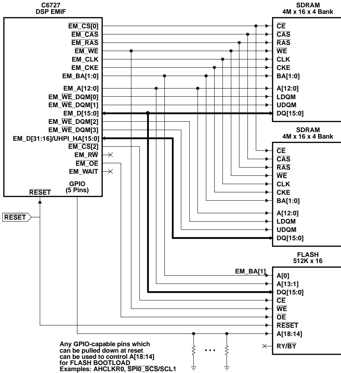
Figure 4-7. C6727 DSP 32-Bit EMIF Example
