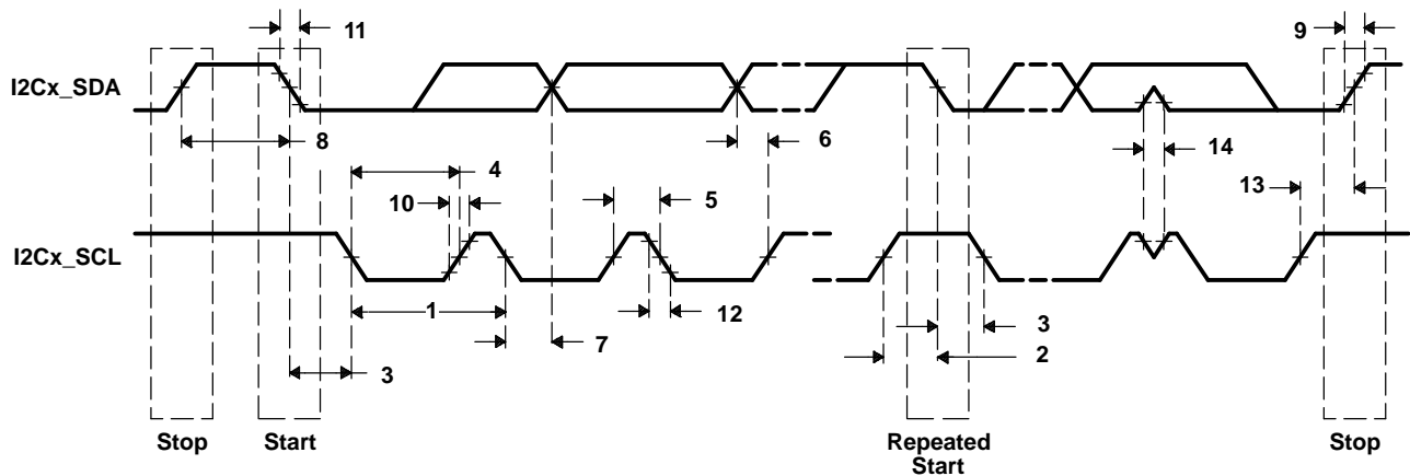
Figure 4-39. I2C Receive Timings
