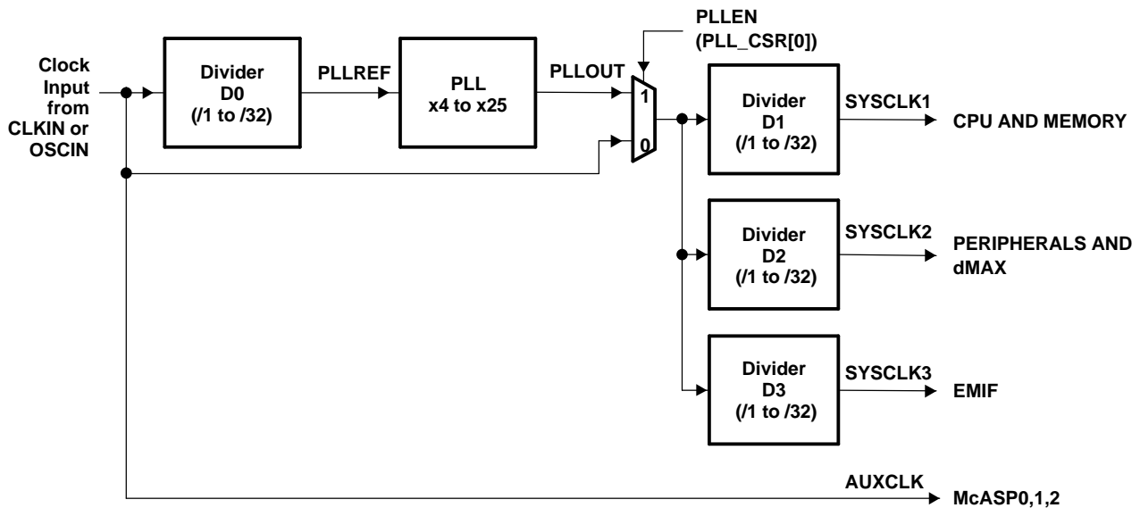
Figure 4-44. PLL Topology
