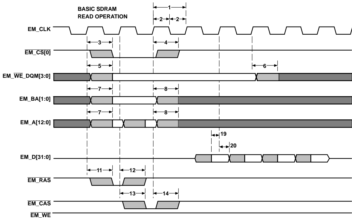
Figure 4-9. Basic SDRAM Read Operation
