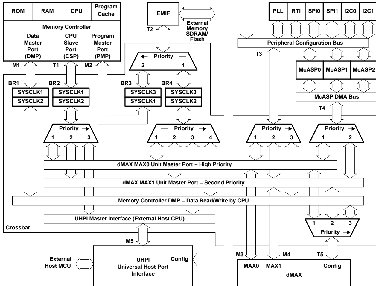
Figure 2-4. Block Diagram of Crossbar Switch
