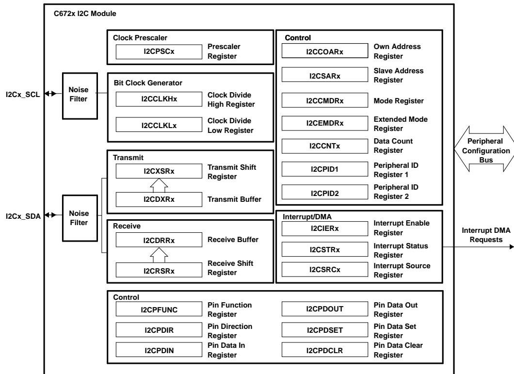
Figure 4-38. I2C Module Block Diagram
