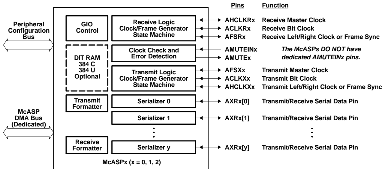
Figure 4-26. McASP Block Diagram
