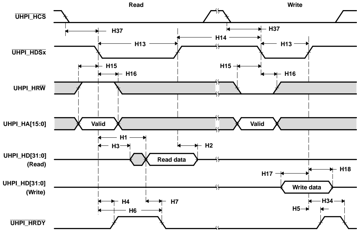
Figure 4-22. Non-Multiplexed Read/Write Timings
