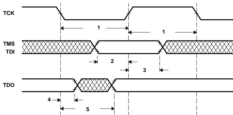
Figure 9. JTAG Scan Timing
