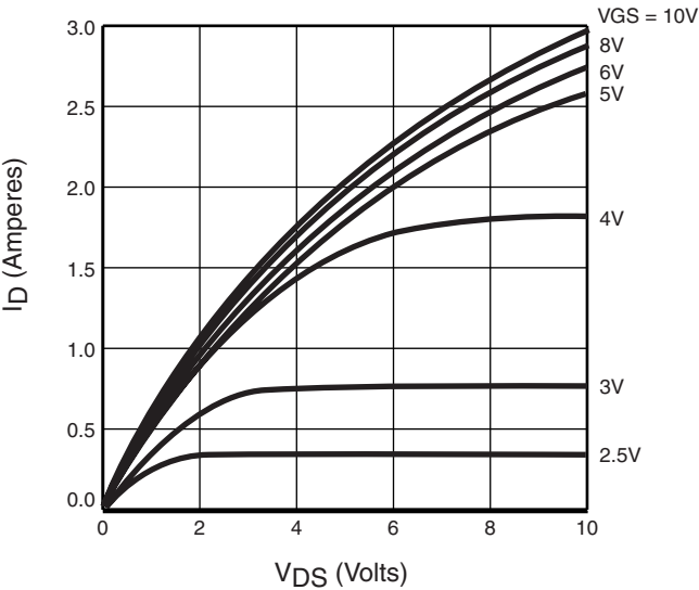
Saturation Characteristics
