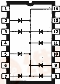
Dwg. No. A-13,359
