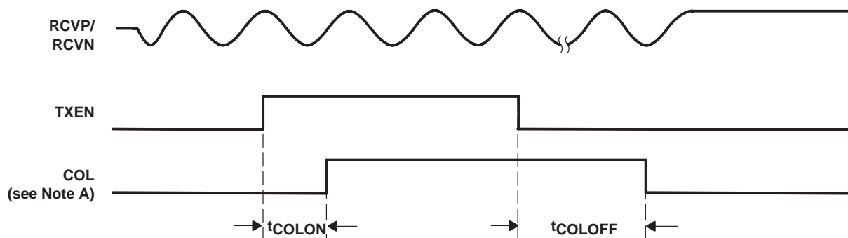
Figure 29. Mode 4 Collision
