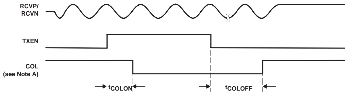
Figure 28. Mode 3 Collision
