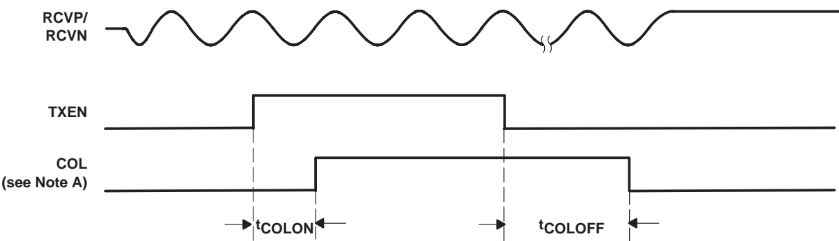
Figure 26. Mode 1 Collision
