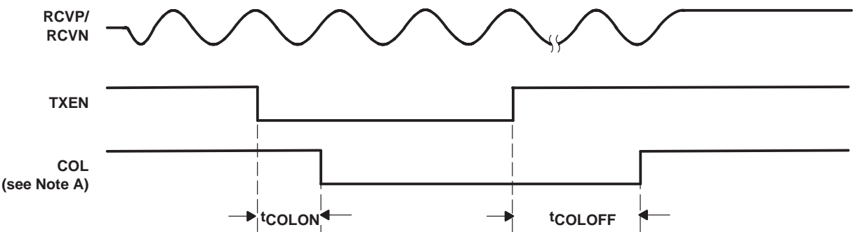
Figure 27. Mode 2 Collision
