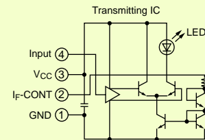
Block diagram of transmission module
