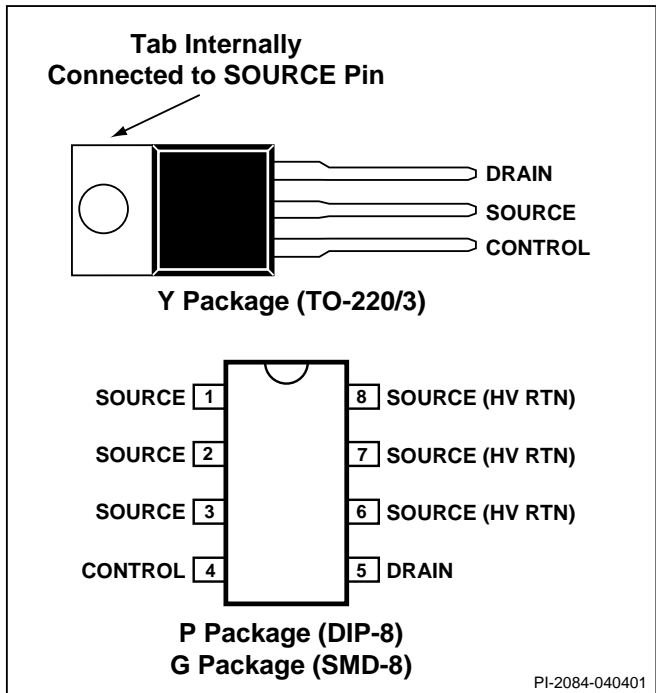
Figure 3. Pin Configuration.
