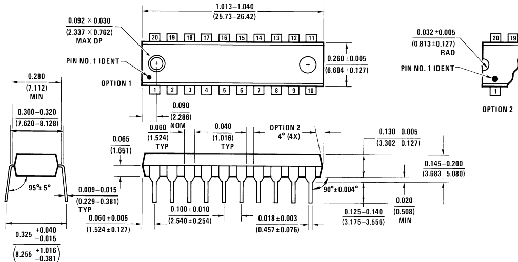
Molded Dual-In-Line Package (N) Order Number TP3420AN NS Package Number N20A
