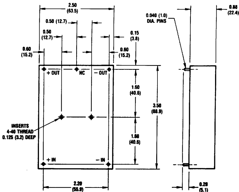
Bottom View
