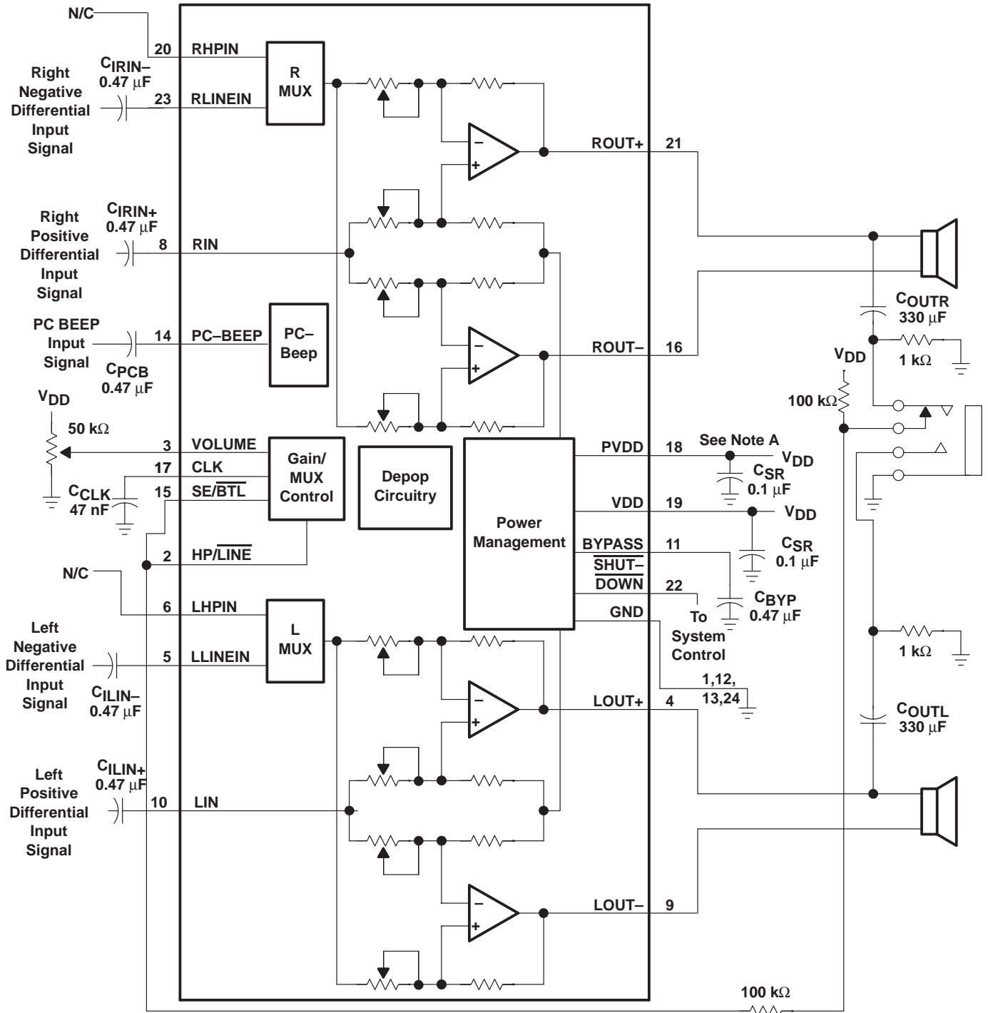
Figure 31. Typical TPA0242 Application Circuit Using Differential Inputs
