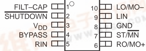
DGQ PACKAGE (TOP VIEW)
