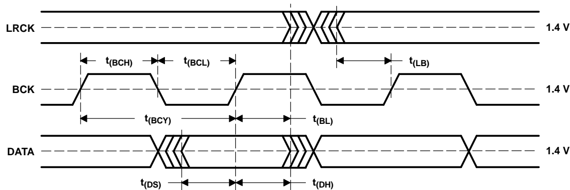
Figure 17. Audio Interface Timing
