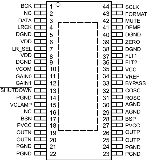
DCP (TOP VIEW)
