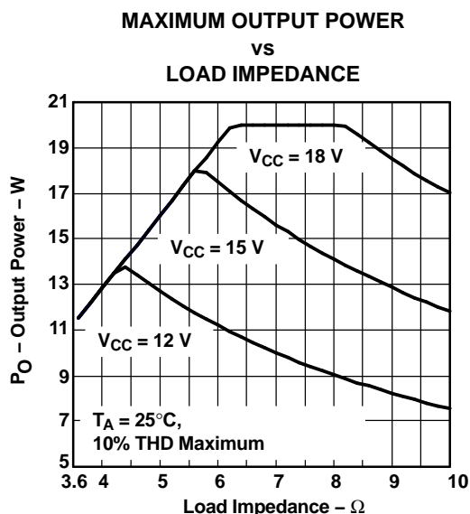
Figure 21. Output Power
