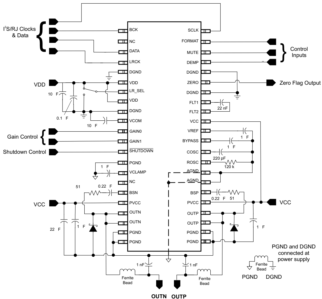
Figure 15. Typical Application Circuit
