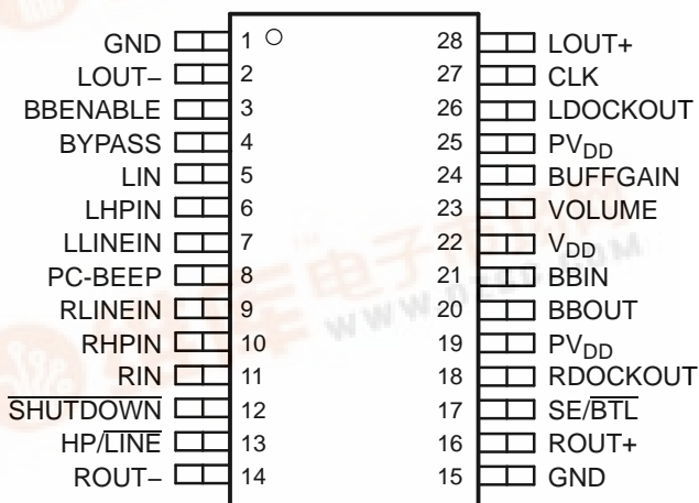
PWP PACKAGE (TOP VIEW)
