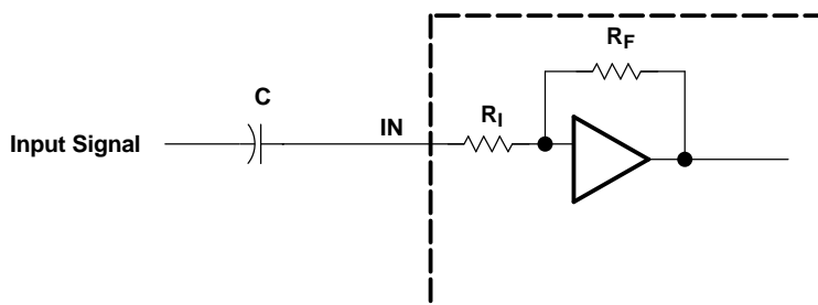
Figure 9. Resistor-On Input for Cut-Off Frequency
