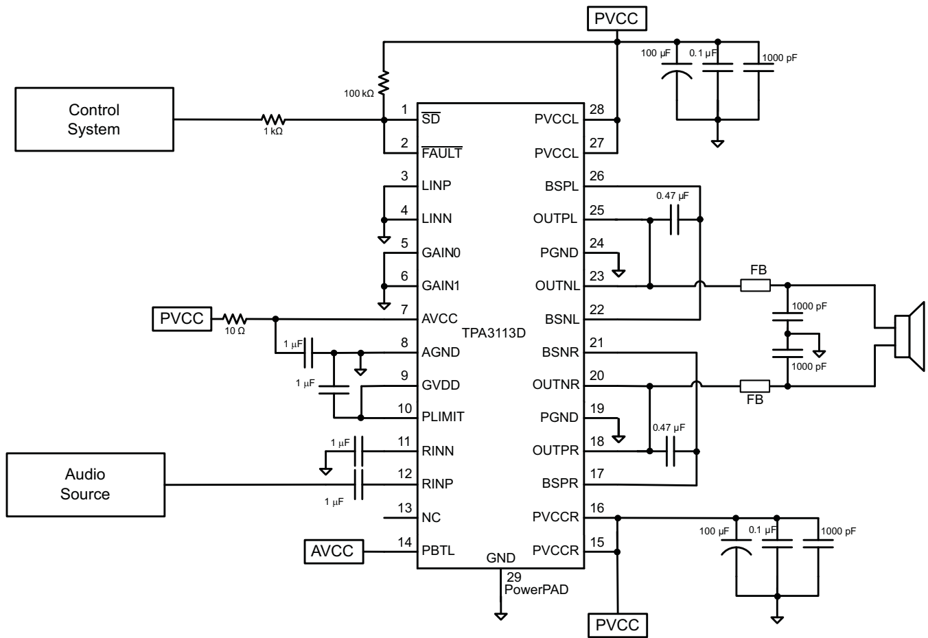
Figure 34. Stereo Class-D Amplifier with PBTl Output and Single-Ended Input
