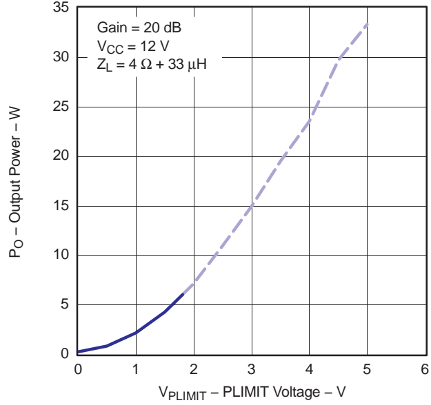
OUTPUT POWER vs PLIMIT VOLTAGE (BTL)
