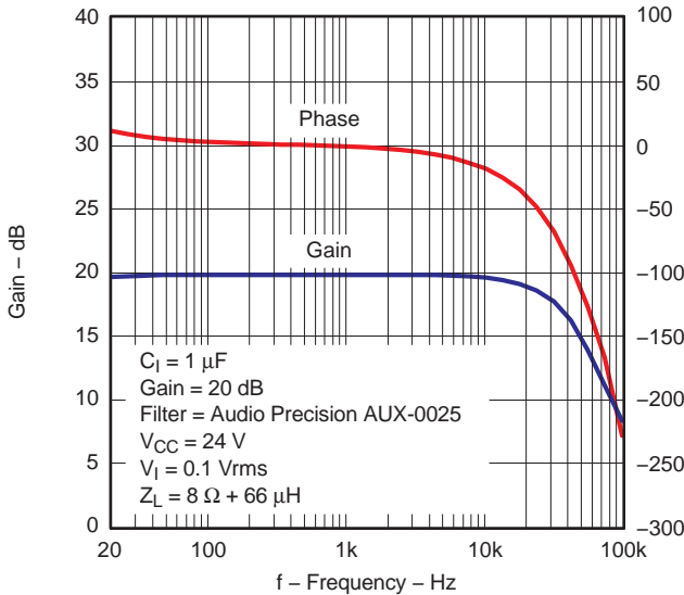
GAIN/PHASE vs FREQUENCY (PBTL)
