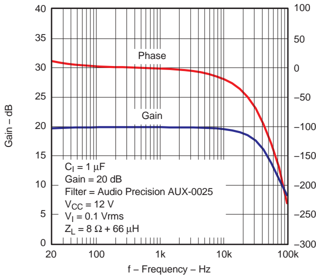
GAIN/PHASE vs FREQUENCY (BTL)
