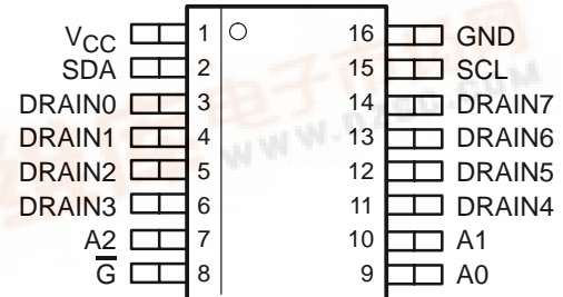
D PACKAGE (TOP VIEW)
