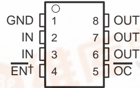
TPS2041A, TPS2051A D PACKAGE (TOP VIEW)
