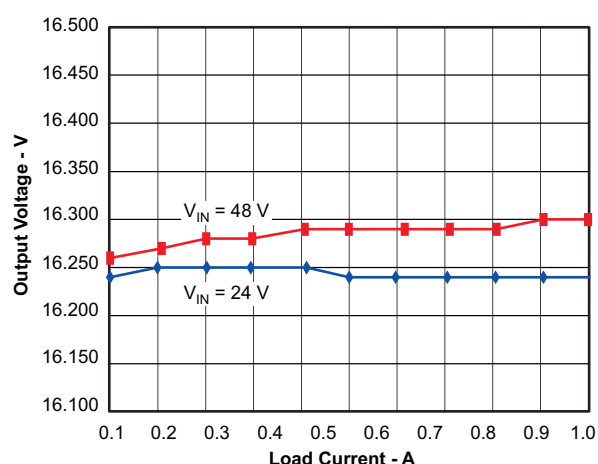
Figure 49. Load Regulation, Two Input Voltage Extremes
