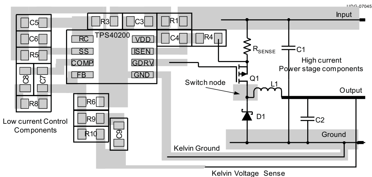
Figure 52. PC Board Layout Recommendations
