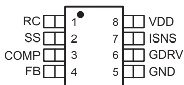
Figure 4. Device Pinout
