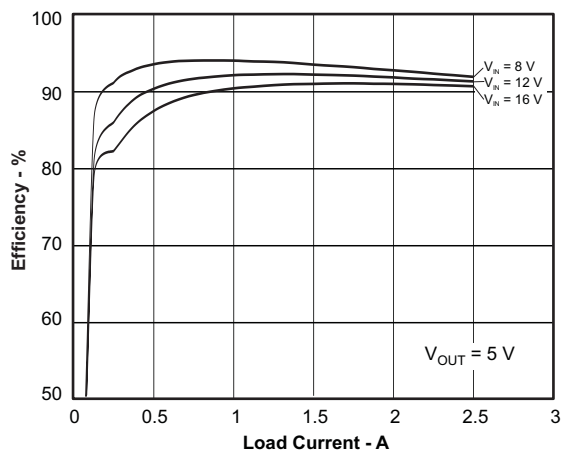
Figure 35. Full-Load Efficiency at 5.0 V OUT
