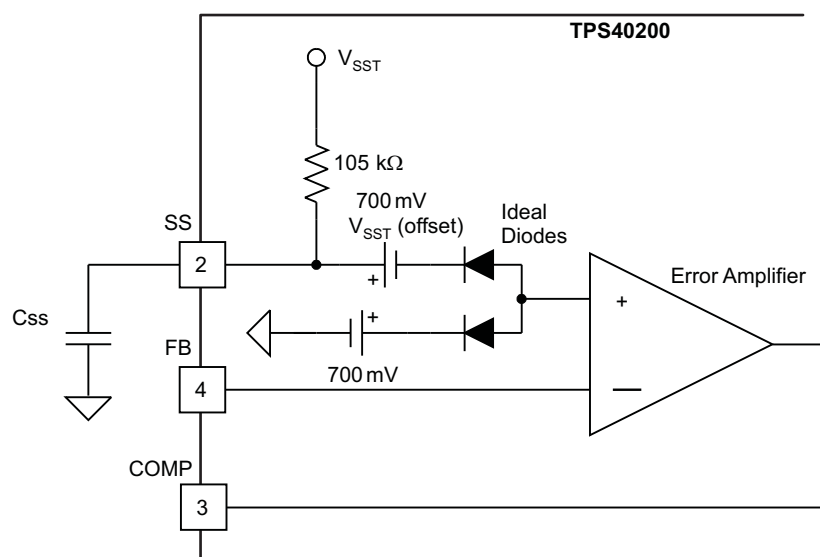
Figure 32. Soft-Start Circuit
