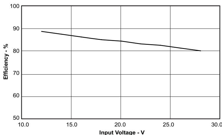
Figure 51. Efficiency vs Input Voltage
