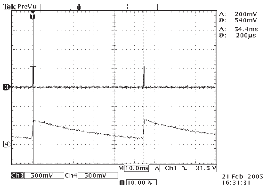
Figure 28. Typical Soft-Start Capacitor and V OUT During Overcurrent
