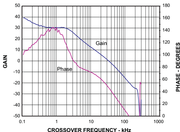
Figure 43. Overall System Gain and Phase Response
