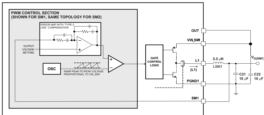
Figure 42. PWM Operation
