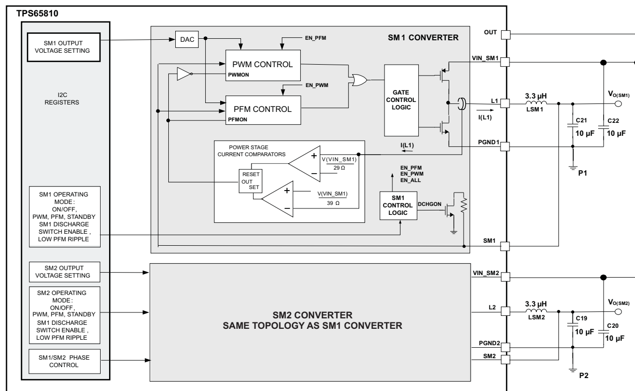
Figure 41. SM1/SM2 Converter
