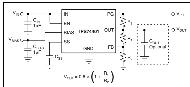
Figure 27. Typical Application Circuit for the TPS74401 (Adjustable)
