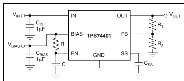
Figure 30. Soft-Start Delay Using an RC Circuit on Enable
