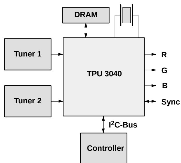
Fig. 2–4: Stand-Alone Application
