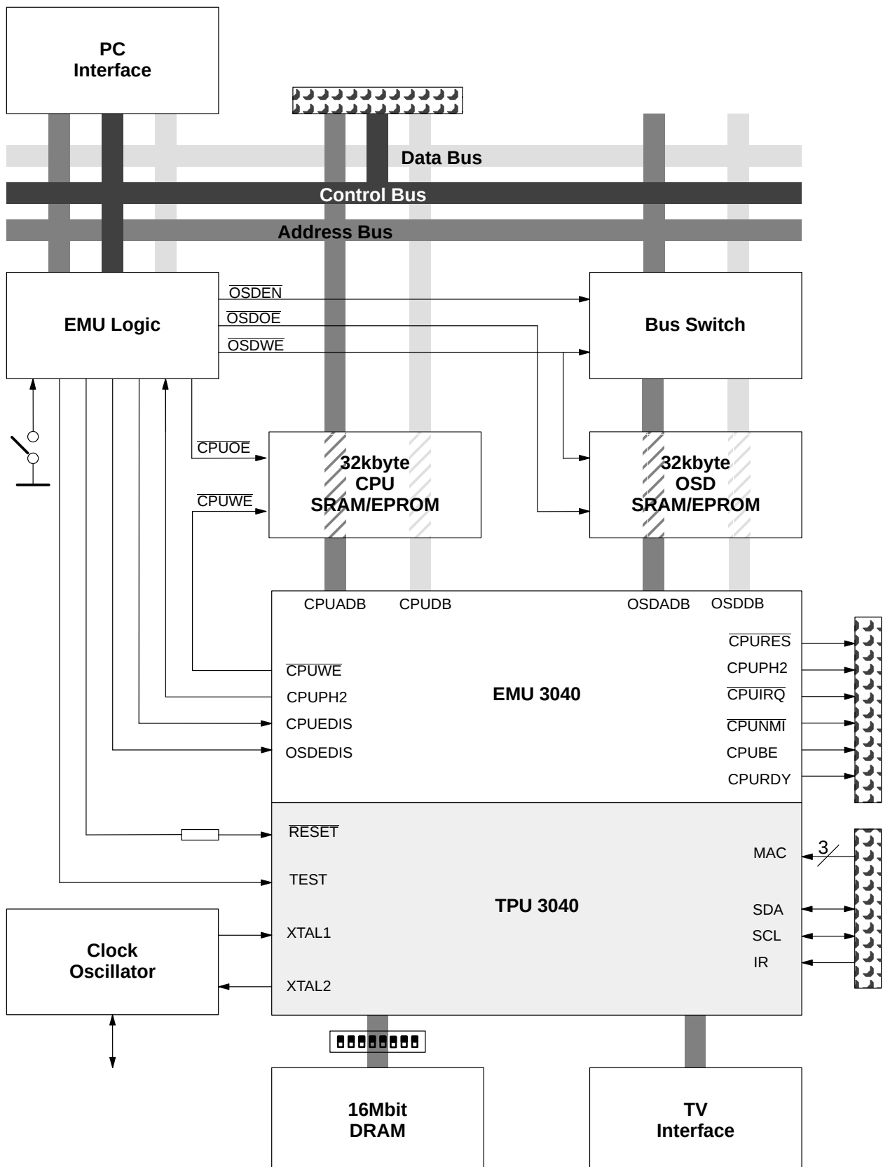
Fig. 6-2: EMU 3040 Board
