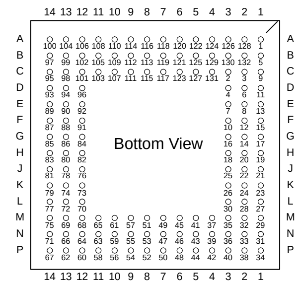
Fig. 6-1: EMU 3040 in 132-pin PGA package
