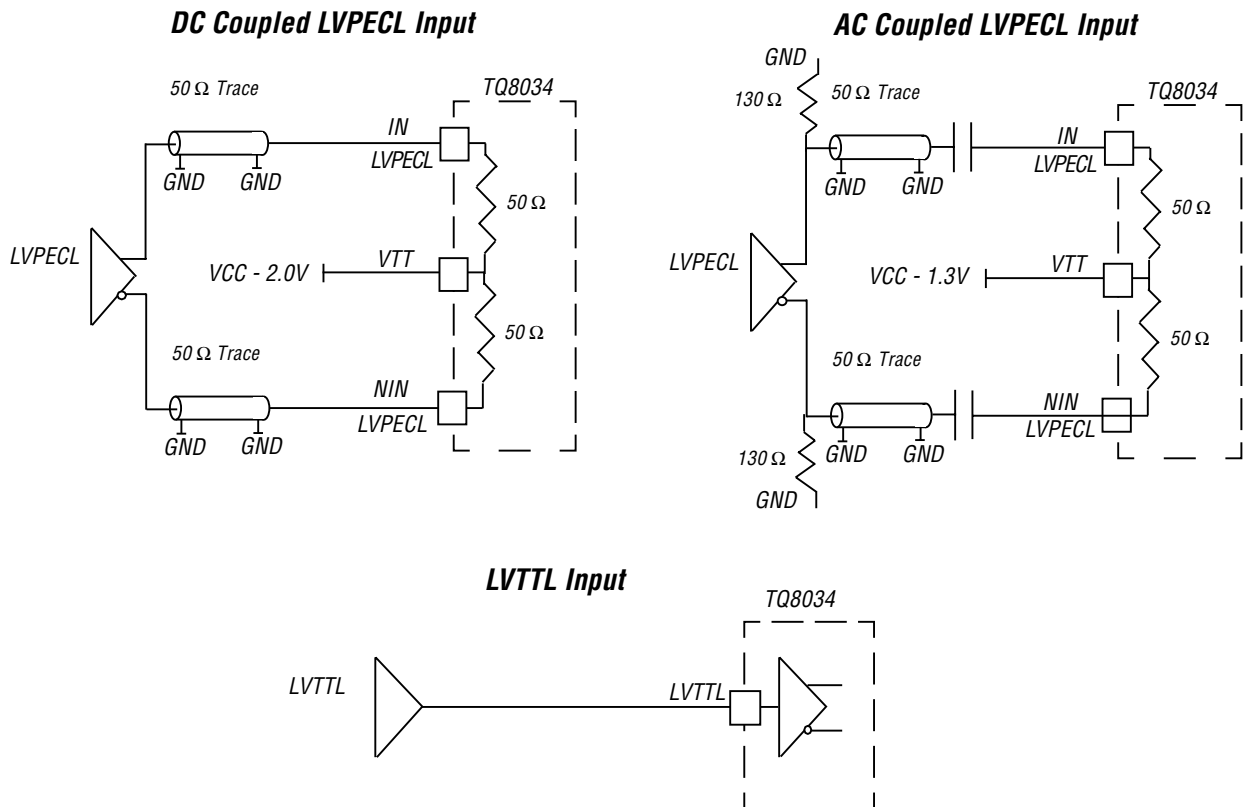
Figure 7. Interface Circuits
