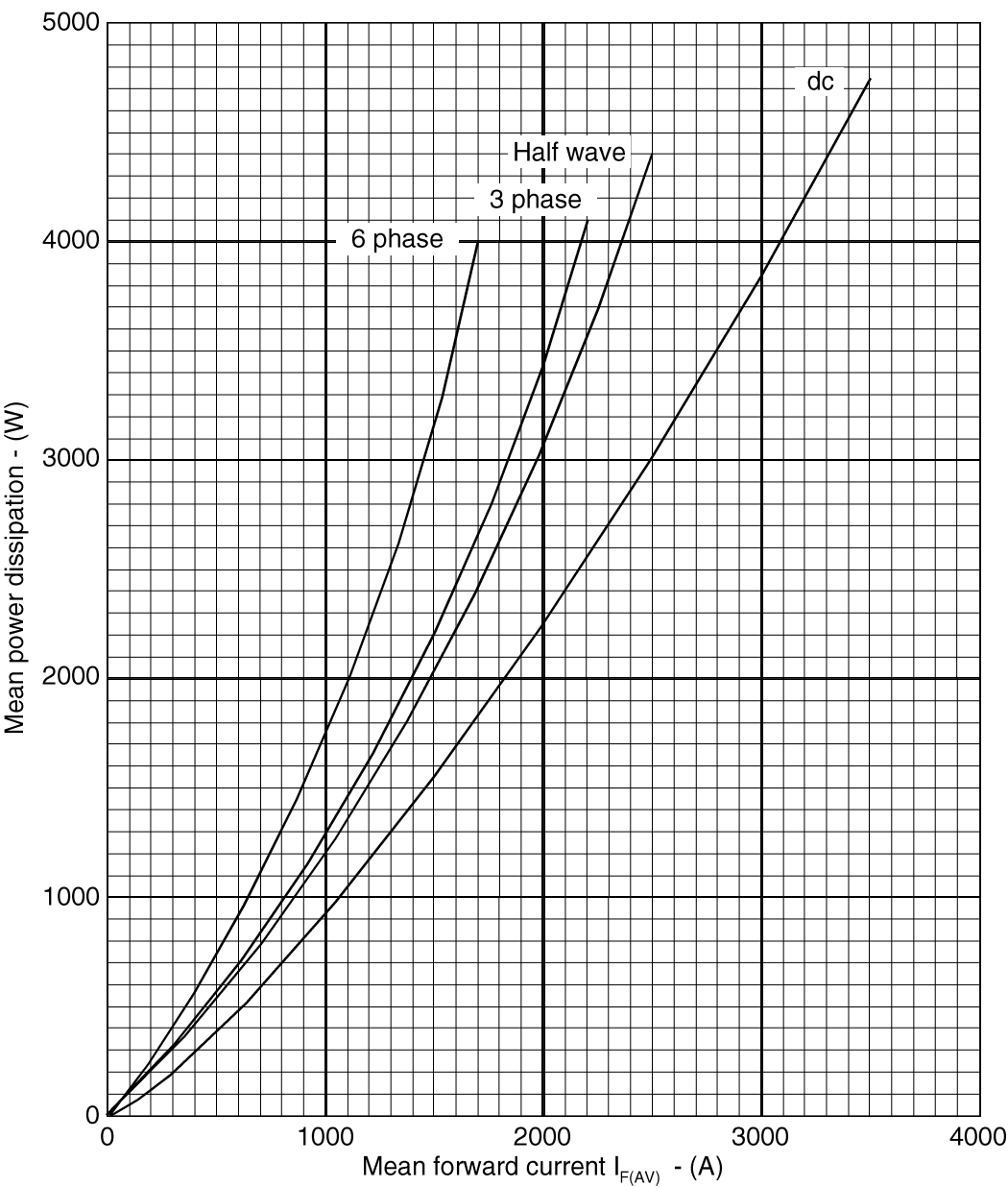
Fig.2 Dissipation curves
