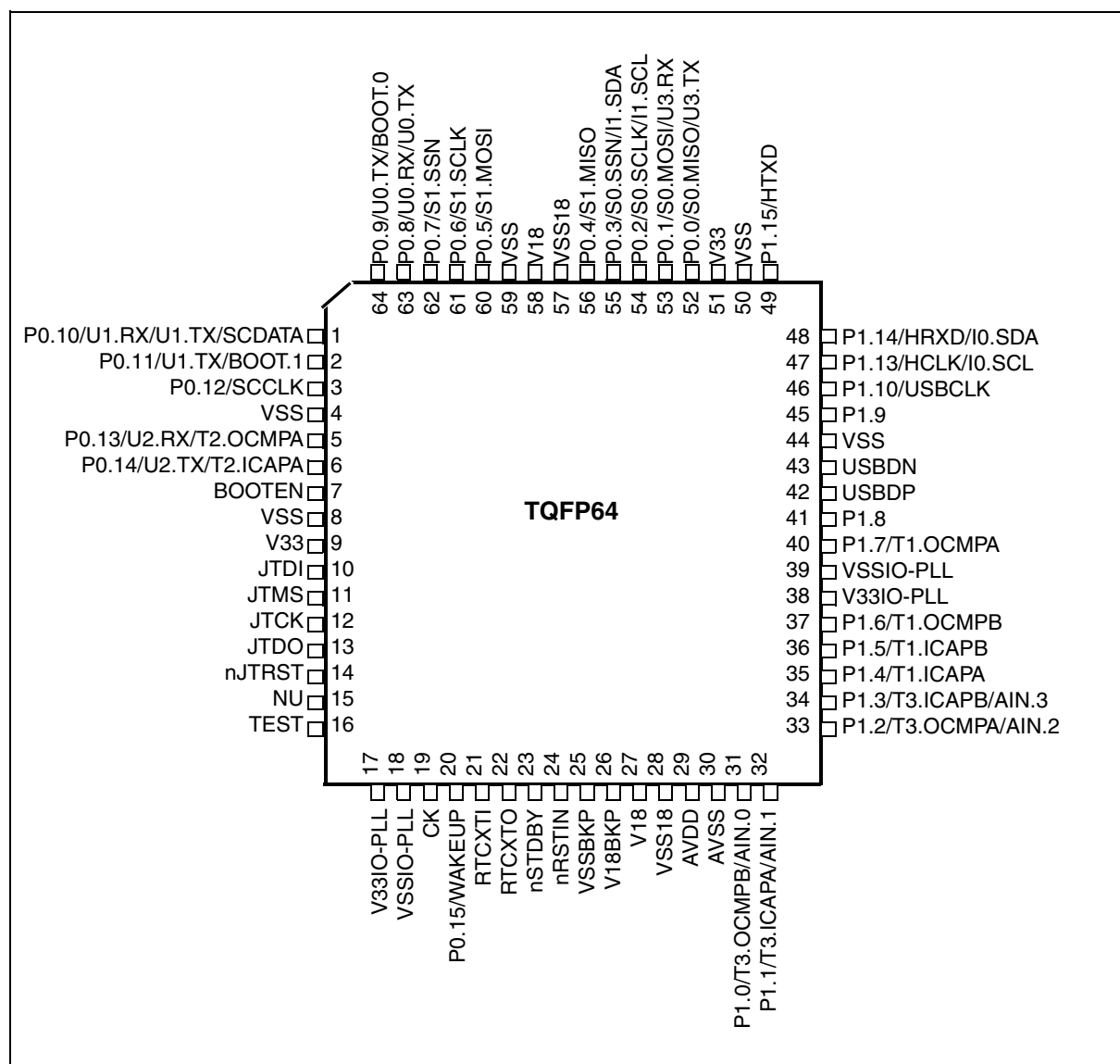
Figure 4. STR711F TQFP64 Pinout
