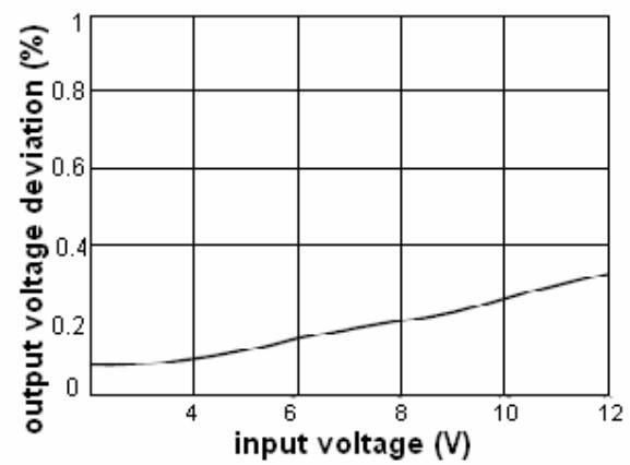
Figure 4: line regulation
