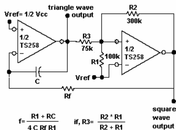
Figure 12. function generator
