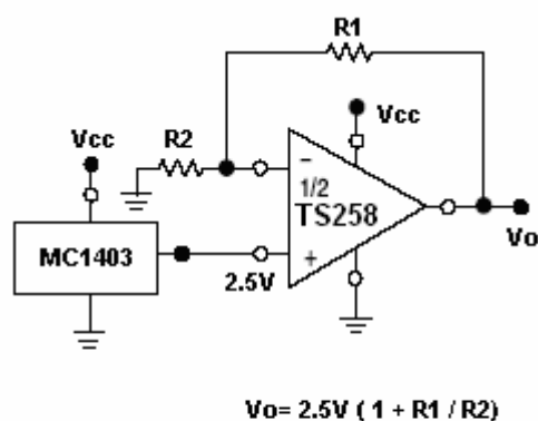
Figure 7. voltage reference
