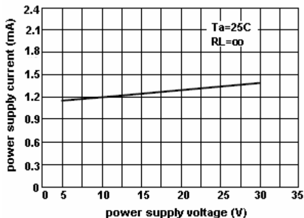
Figure 6. power supply current vs supply voltage
