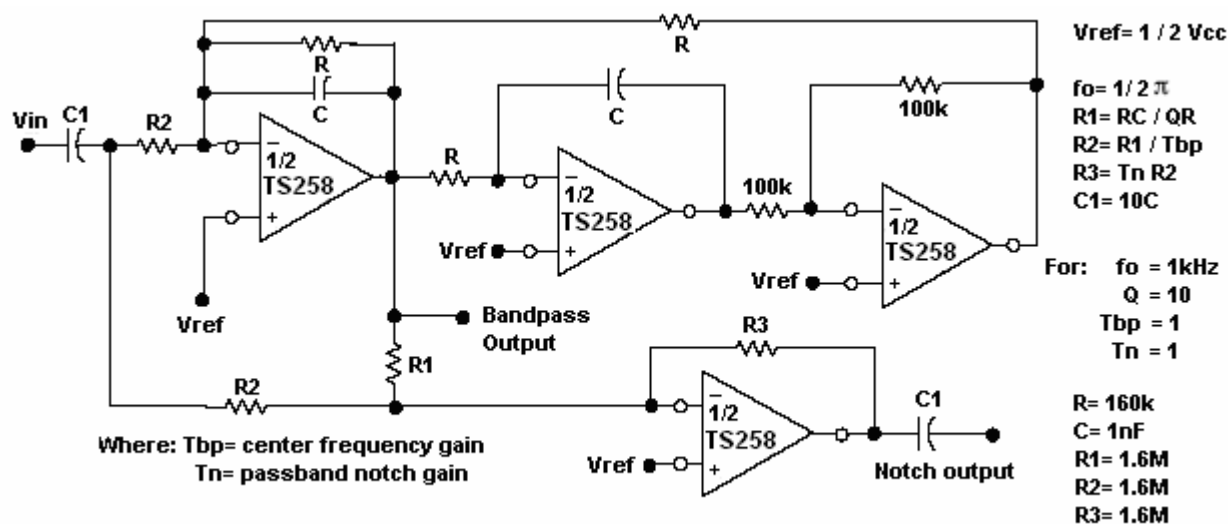
Figure 9. bi-quad filter
