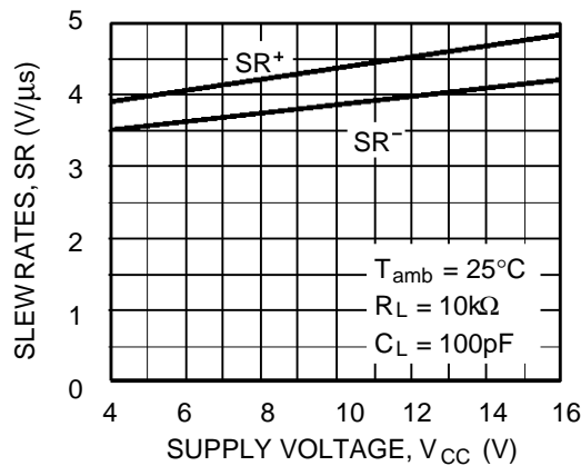
Figure 28 : Slew Rates versus Supply Voltage
