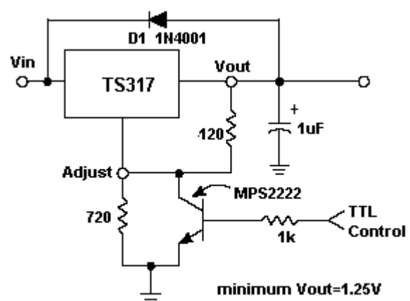
D1 protects the device an input short circuit
