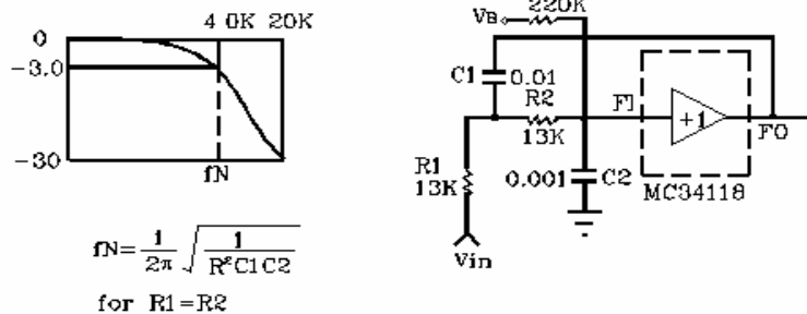
Figure 9. Low Pass Filter
