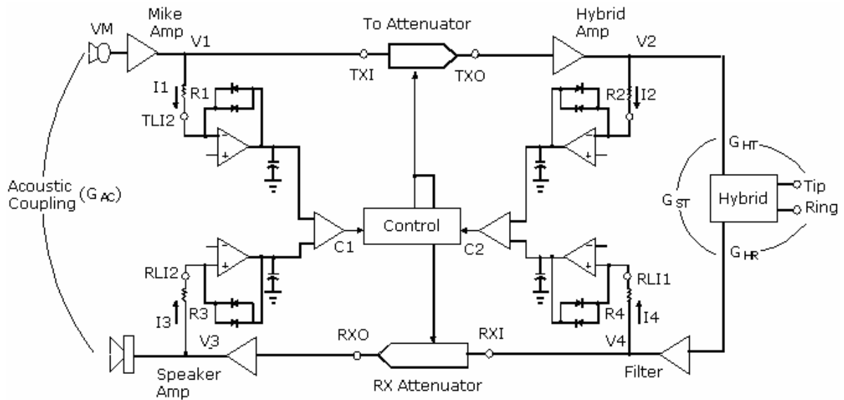
Figure 10. Basic Block Diagram For Design Purpos
