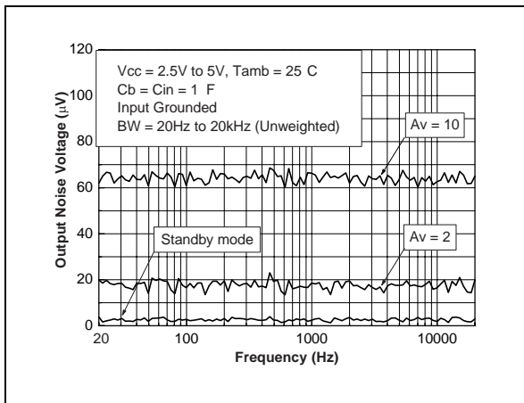
Fig. 79 : Vout1+Vout2 Unweighted Noise Floor
