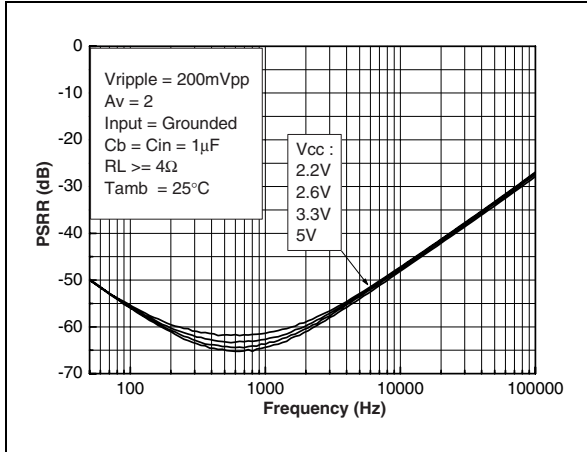
Figure 9: Power supply rejection ratio (PSRR) vs. frequency
