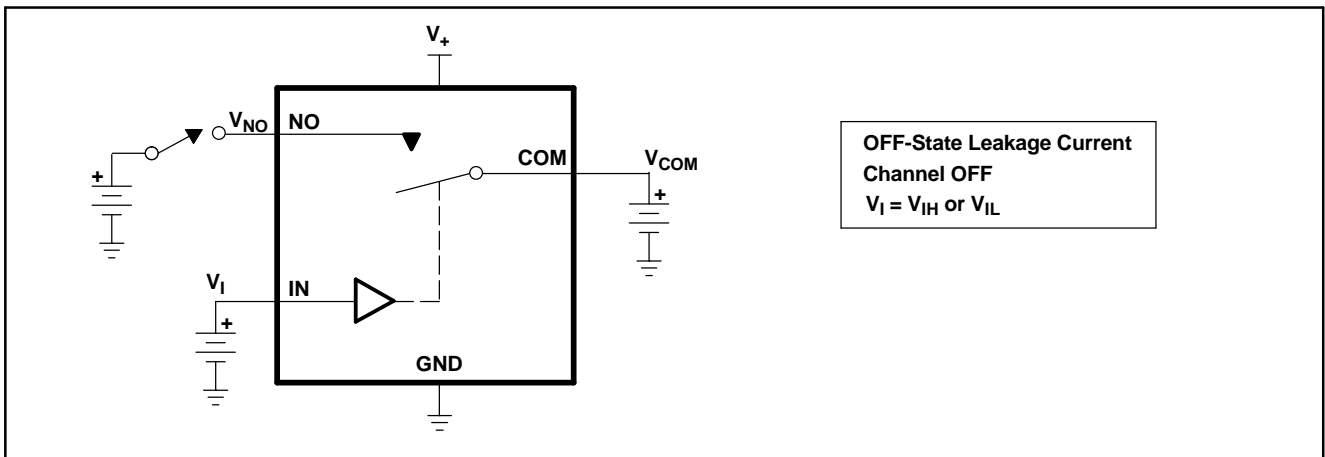
Figure 14. OFF-State Leakage Current ( I_{COM(OFF)} , I_{NC(OFF)} , I_{COM(PWROFF)} , I_{NC(PWRFF)} )
