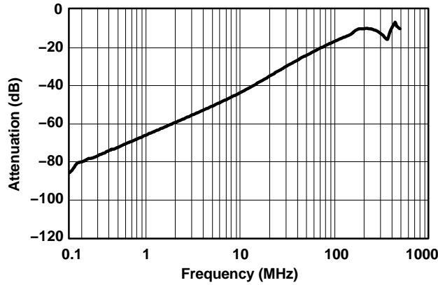
Figure 10. OFF Isolation and Crosstalk ( V_+ = 5\text{ V} )
