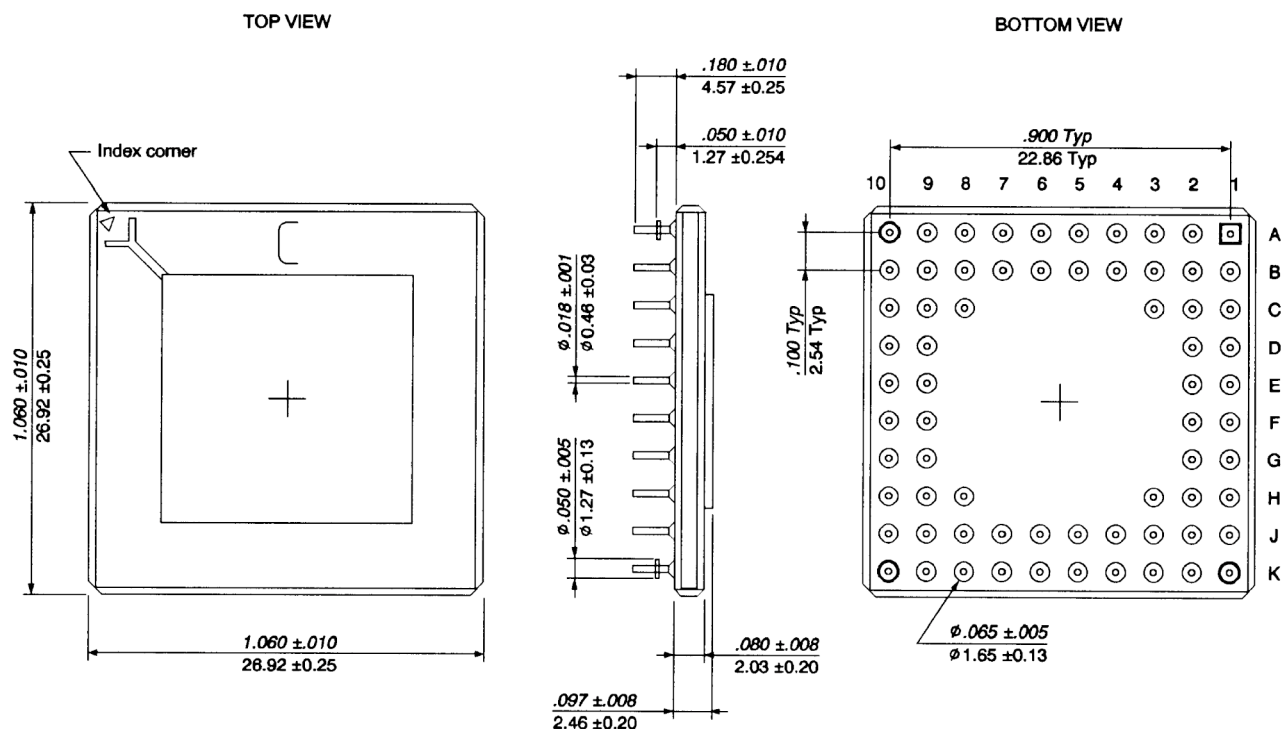
Figure 23. 68-lead CPGA
