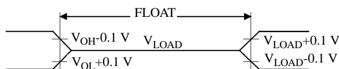
Figure 19. Float Waveforms
