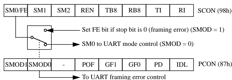
Figure 4. Framing Error Block Diagram
