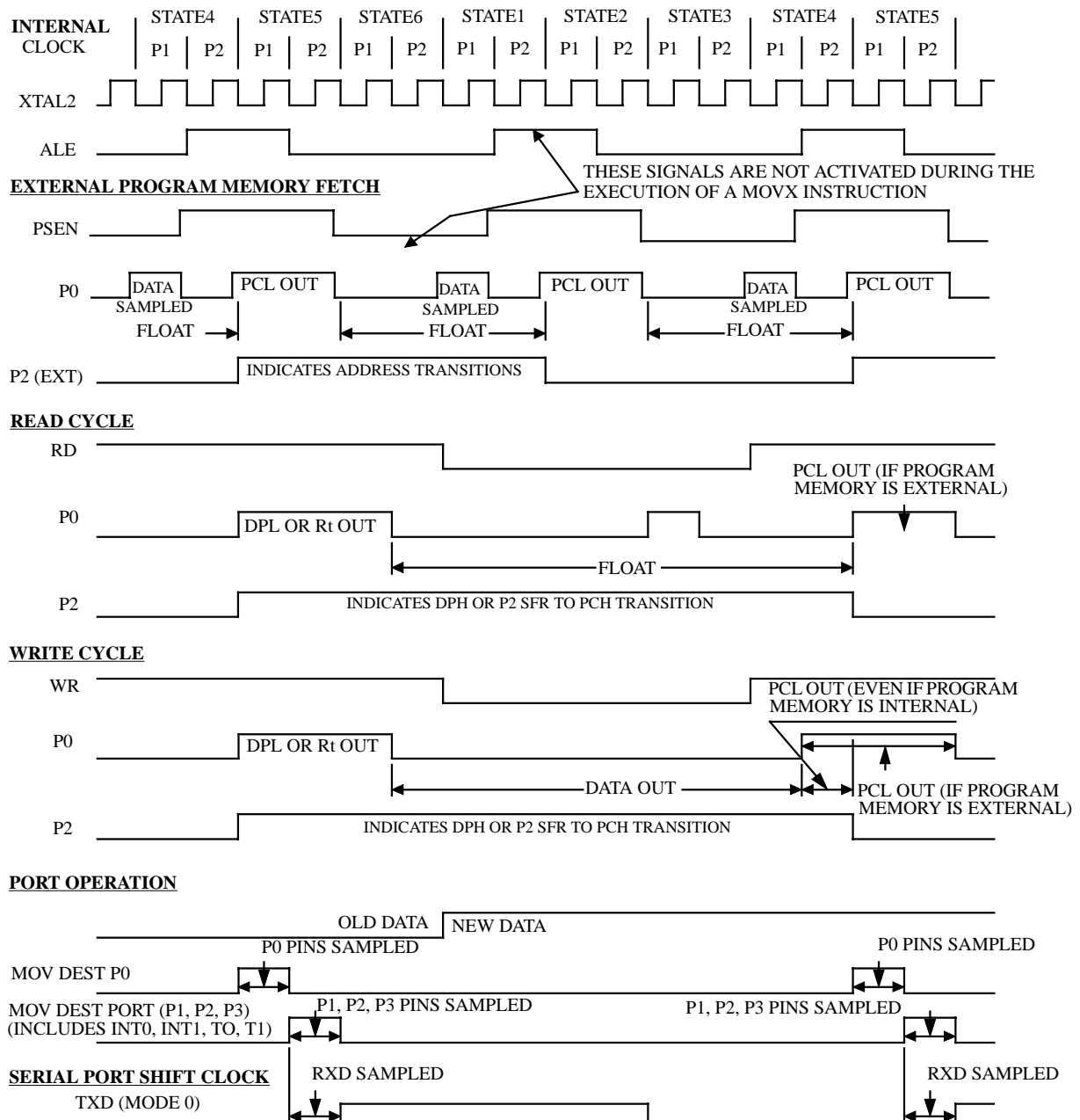
Figure 20. Clock Waveforms
