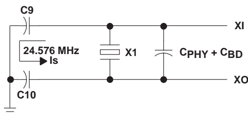
Figure 11. Load Capacitance for the TSB41LV06A PHY
