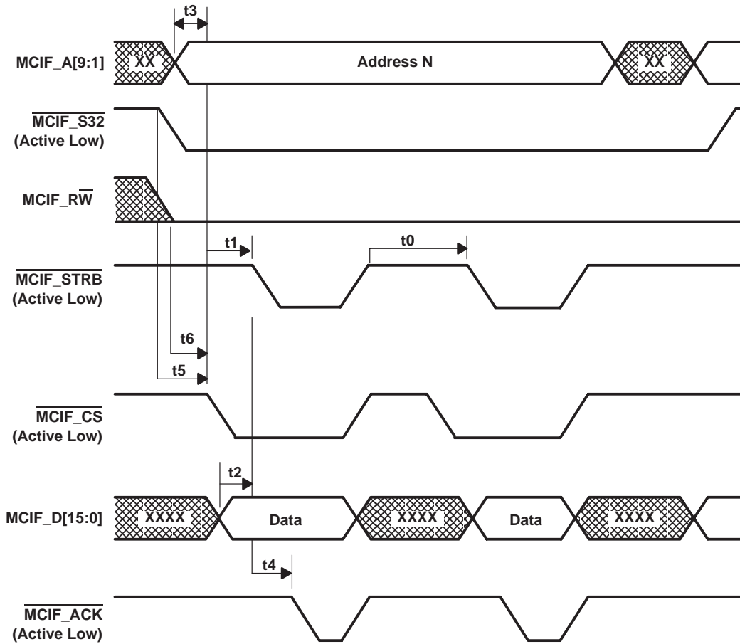
Figure 3–6. Microcontroller Interface Critical Write Timing
