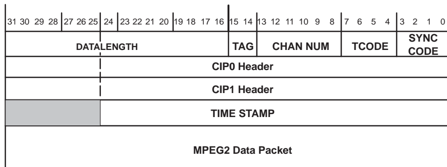
Figure 5–12. MPEG2 Receive Format
