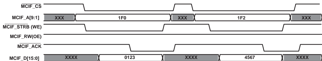
Figure 3–9. Host Port Multistrobe Timing – Write Operation
