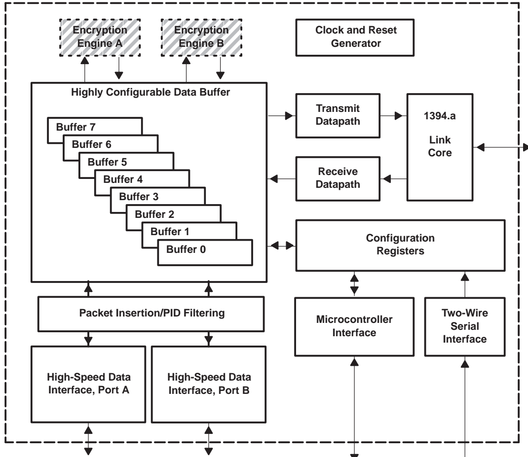
Figure 2-5. ceLynx Functional Block Diagram
