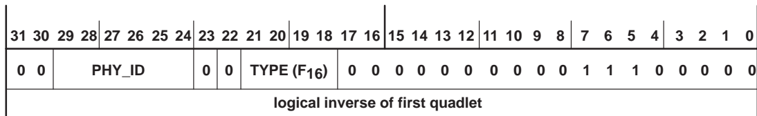
Figure 5–30. Resume Packet
