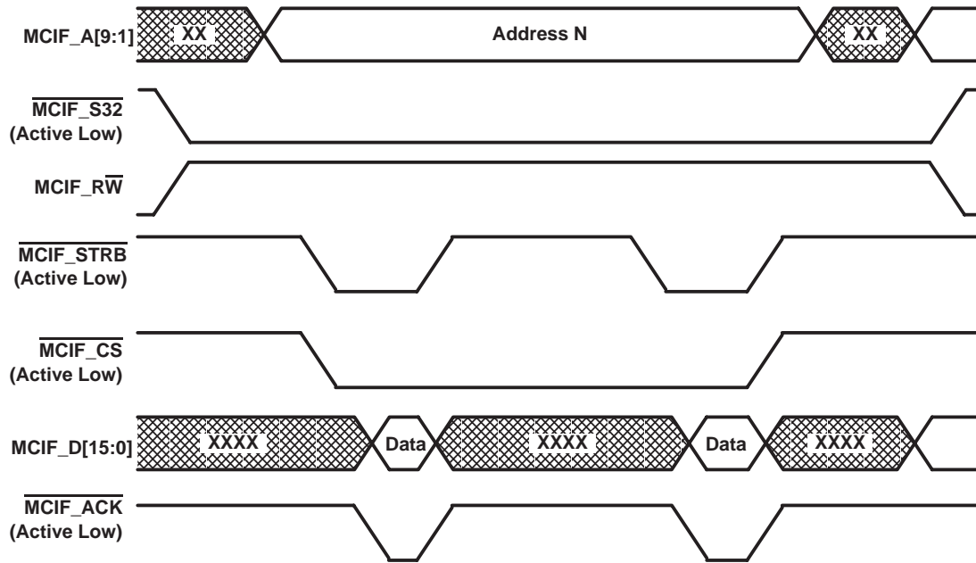
Figure 3–3. 32-Bit Read
