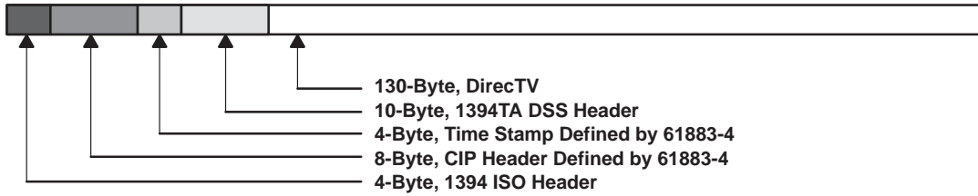
Figure 5-14. 1394 DirectTV Packet
