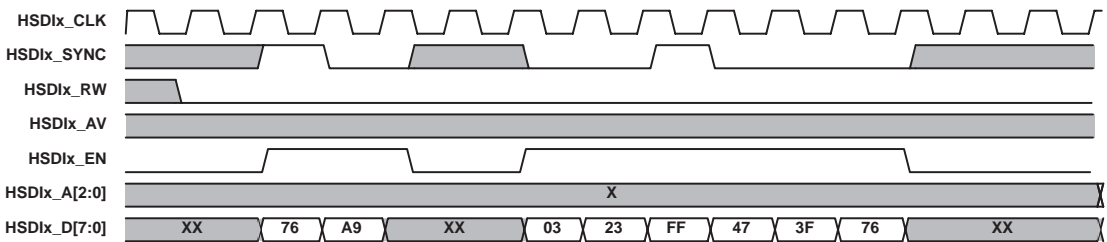
Figure 3–20. HSDI Write, Byte-Wide Data Bus, Sync Mode B
