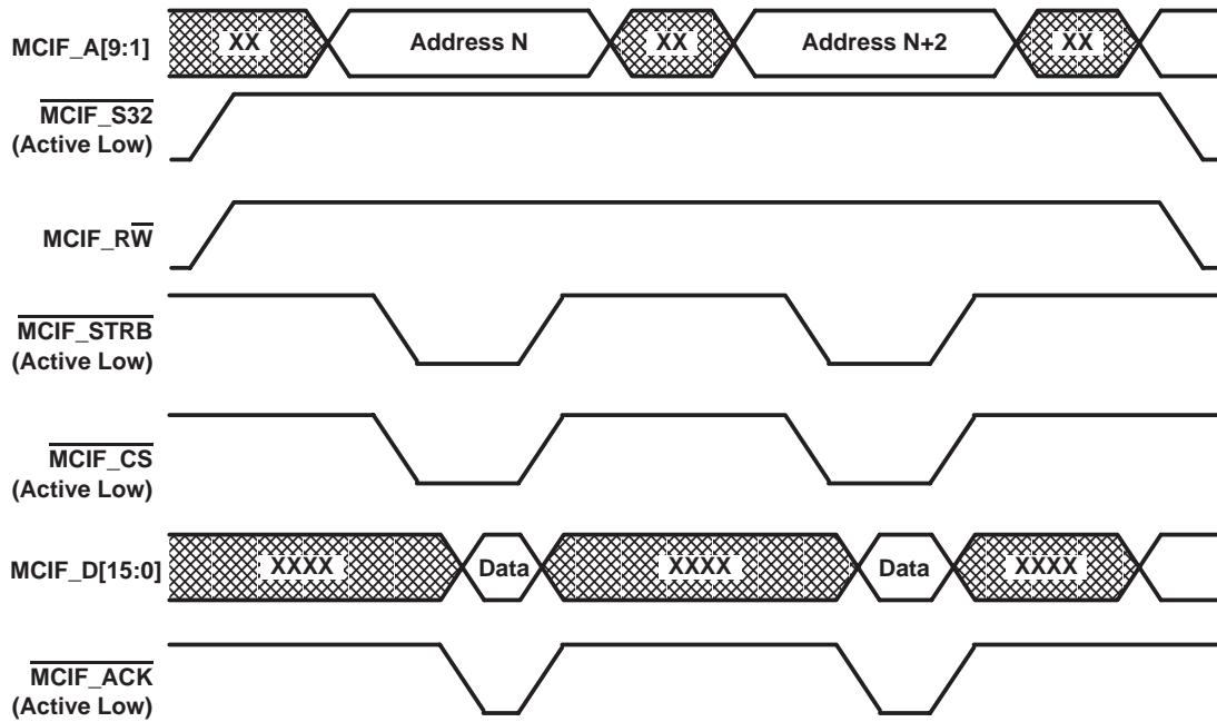
Figure 3–2. 16-Bit Read
