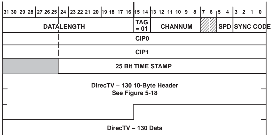
Figure 5-15. DirecTV Transmit Format
