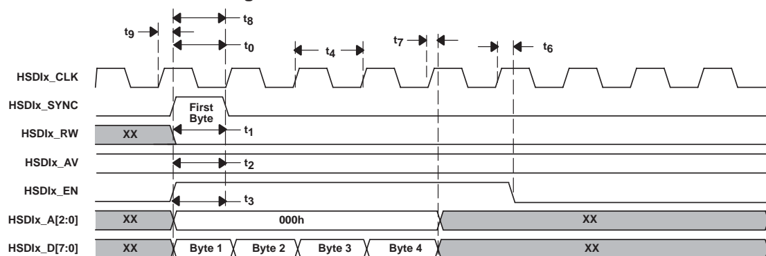
Figure 3–25. HSDI Interface Critical Timing
