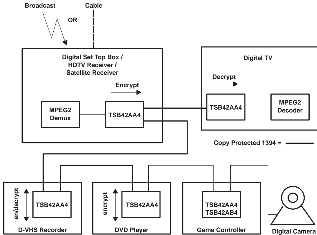
Figure 2-1. Home Entertainment System Interconnect With Content Protection
