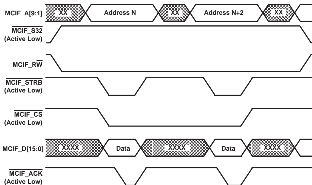
Figure 3–4. 16-Bit Write
