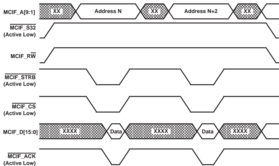
Figure 3–2. 16-Bit Read
