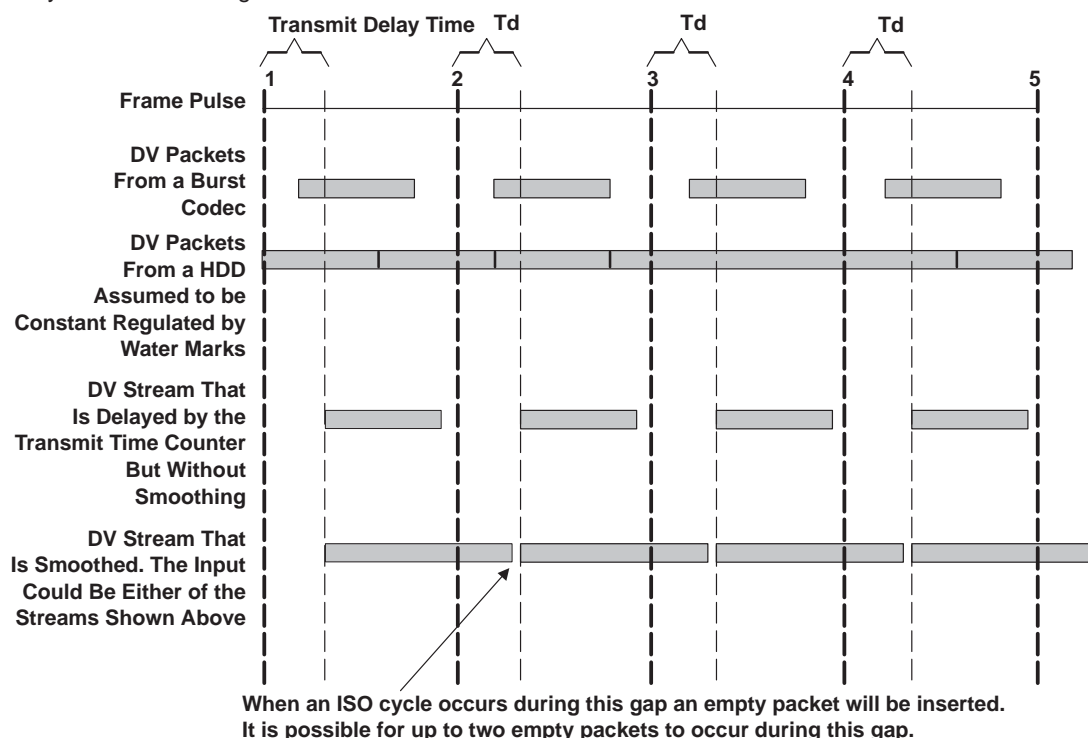
Figure 5-24. DV Smoothing
