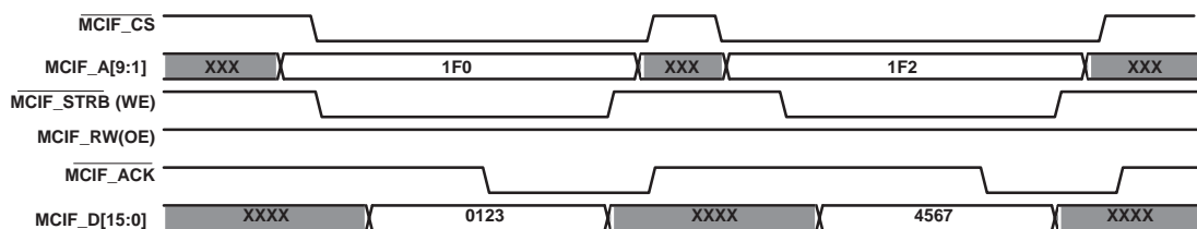
Figure 3–9. Host Port Multistrobe Timing – Write Operation
