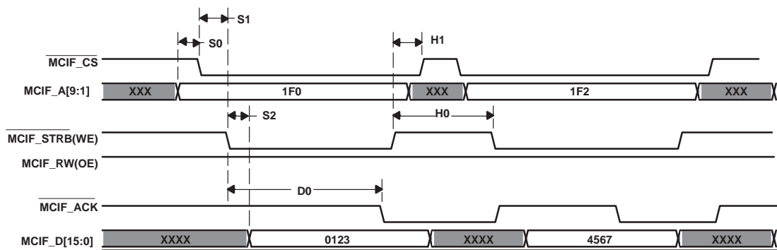
Figure 3-11. Multistrobe Mode – Write Critical Timing
