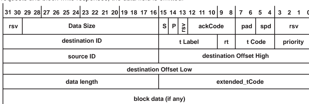
Figure 5–7. Block Receive Format
