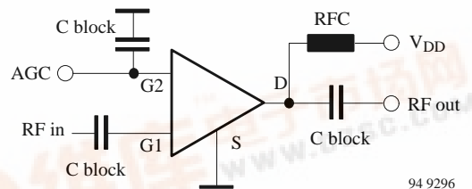
Amplifier 2
