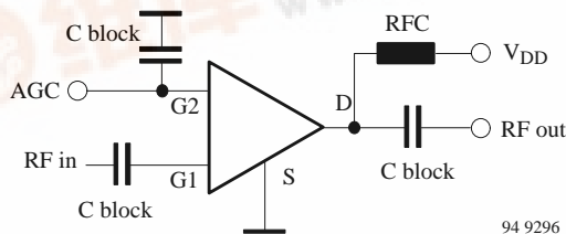
Amplifier 1
