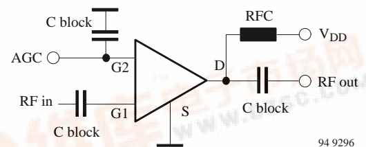
Amplifier 2
