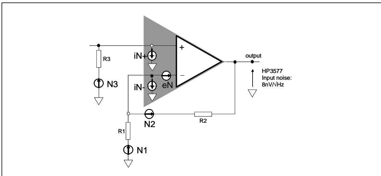
Figure 32: Noise model
