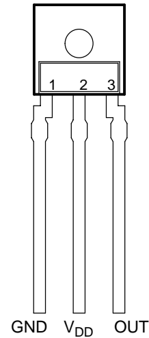
SR PACKAGE (FRONT VIEW)
