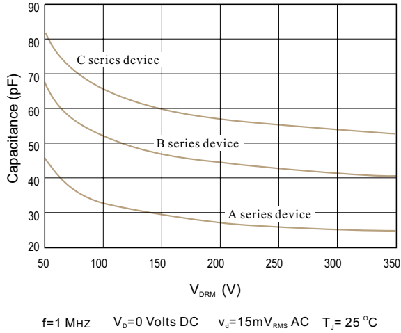
TYPICAL CAPACITANCE V.S. RATED REPETITIVE OFF-STATE VOLTAGE
