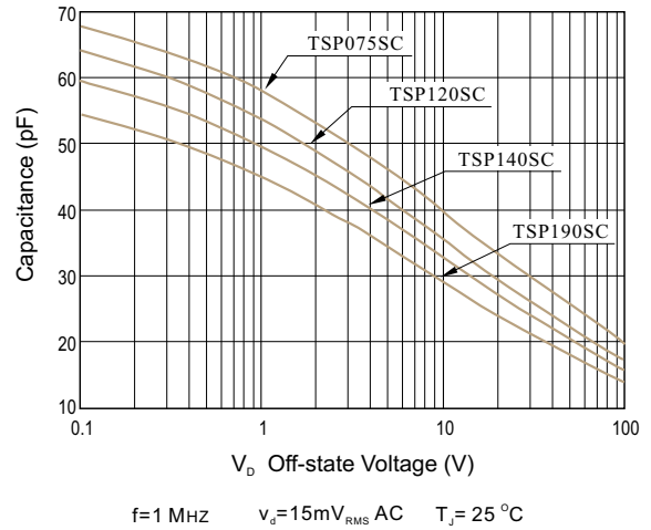
TYPICAL CAPACITANCE V.S. OFF-STATE VOLTAGE
