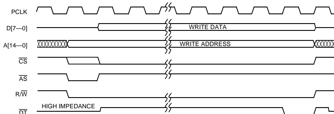
Figure 8. Synchronous Write
