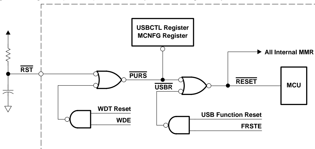
Figure 2–2. Reset Diagram
