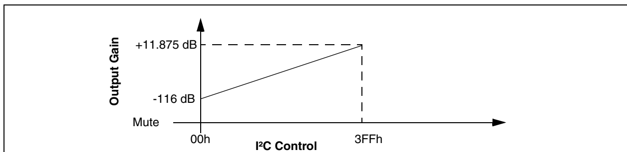
Figure 19: Volume Control
