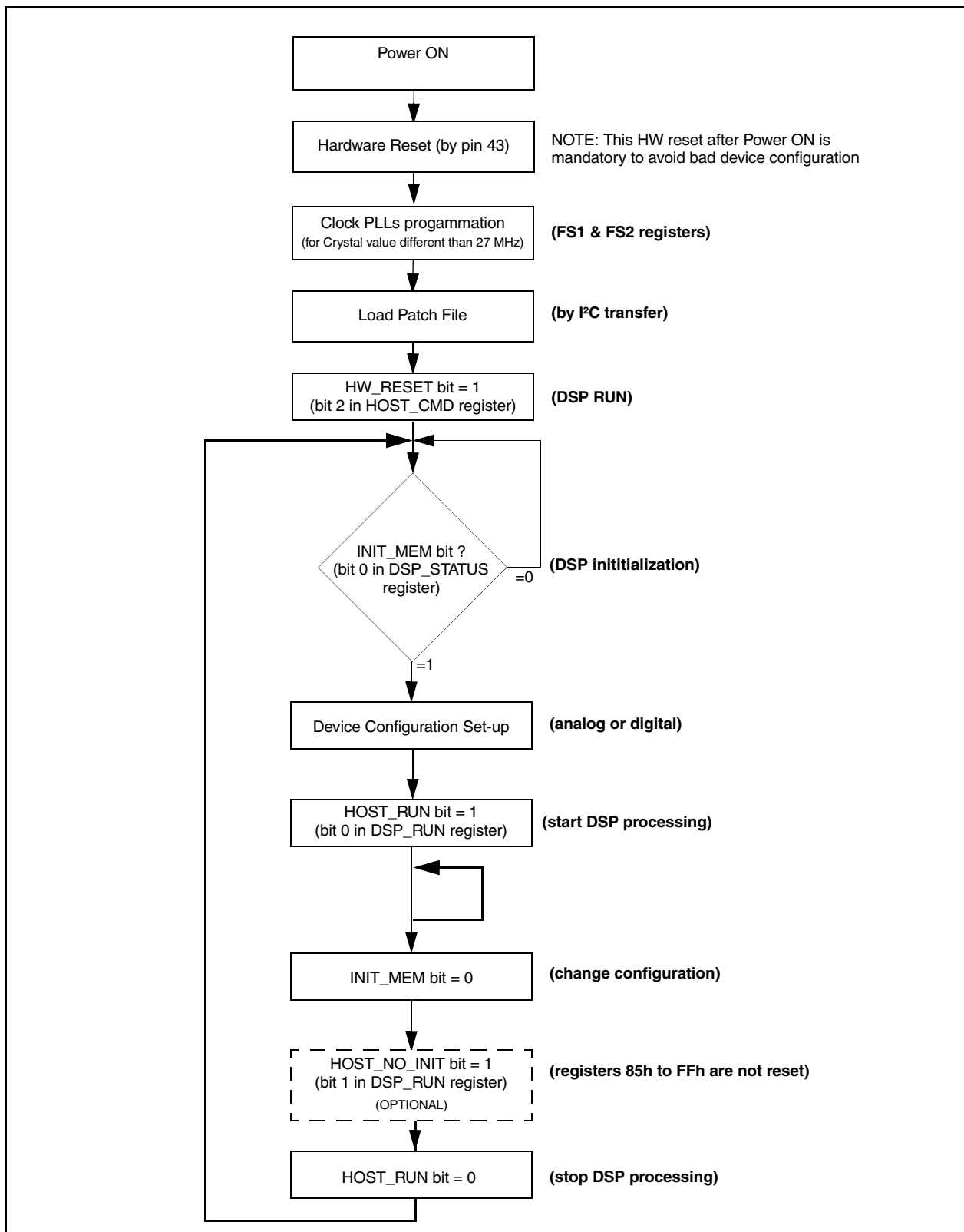
Figure 27: Flow chart
