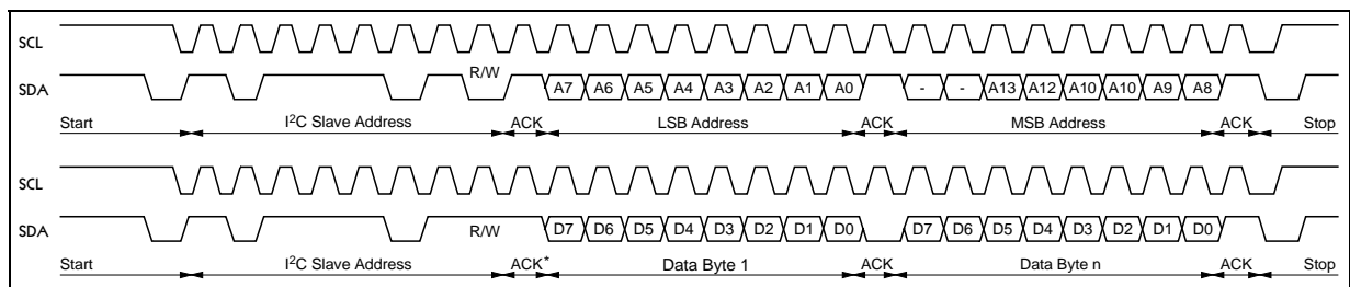
Figure 5 : MCU I 2 C Read Operation
