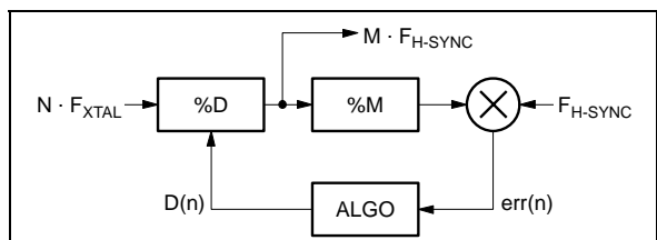
Figure 12 : Digital PLL
