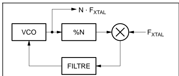
Figure 11 : Analogic PLL
