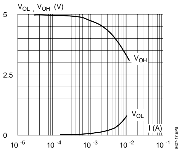
Figure 1 : R, G, B, FBLK Typical Outputs Static Characteristics
