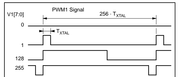
Figure 8 : PWM Timing
