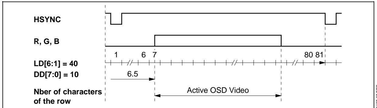
Figure 7 : Horizontal Timing
